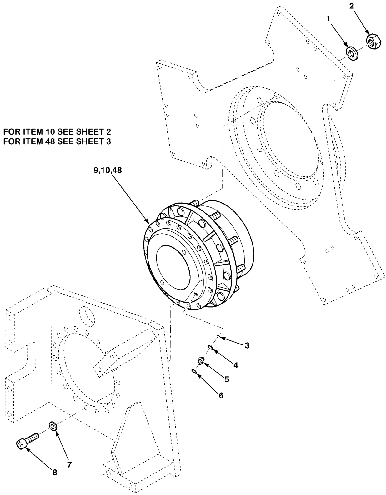
Figure 79. Rear Propel Gearbox Assembly (Sheet 1 of 3)
