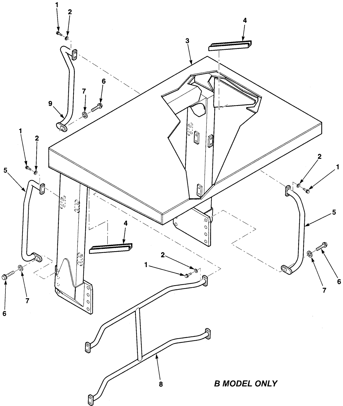
Figure 98. Rollover Protection Structure (ROPS) Assembly and Handrails (Sheet 1 of 2)
