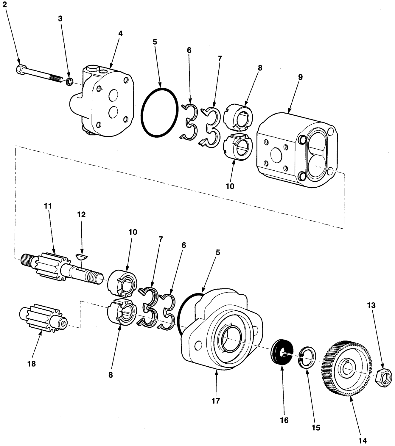
Figure 89. Power Steering Pump
