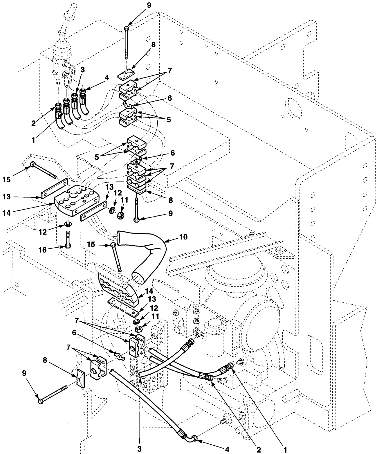
Figure 126. Pilot Lines and Fittings
