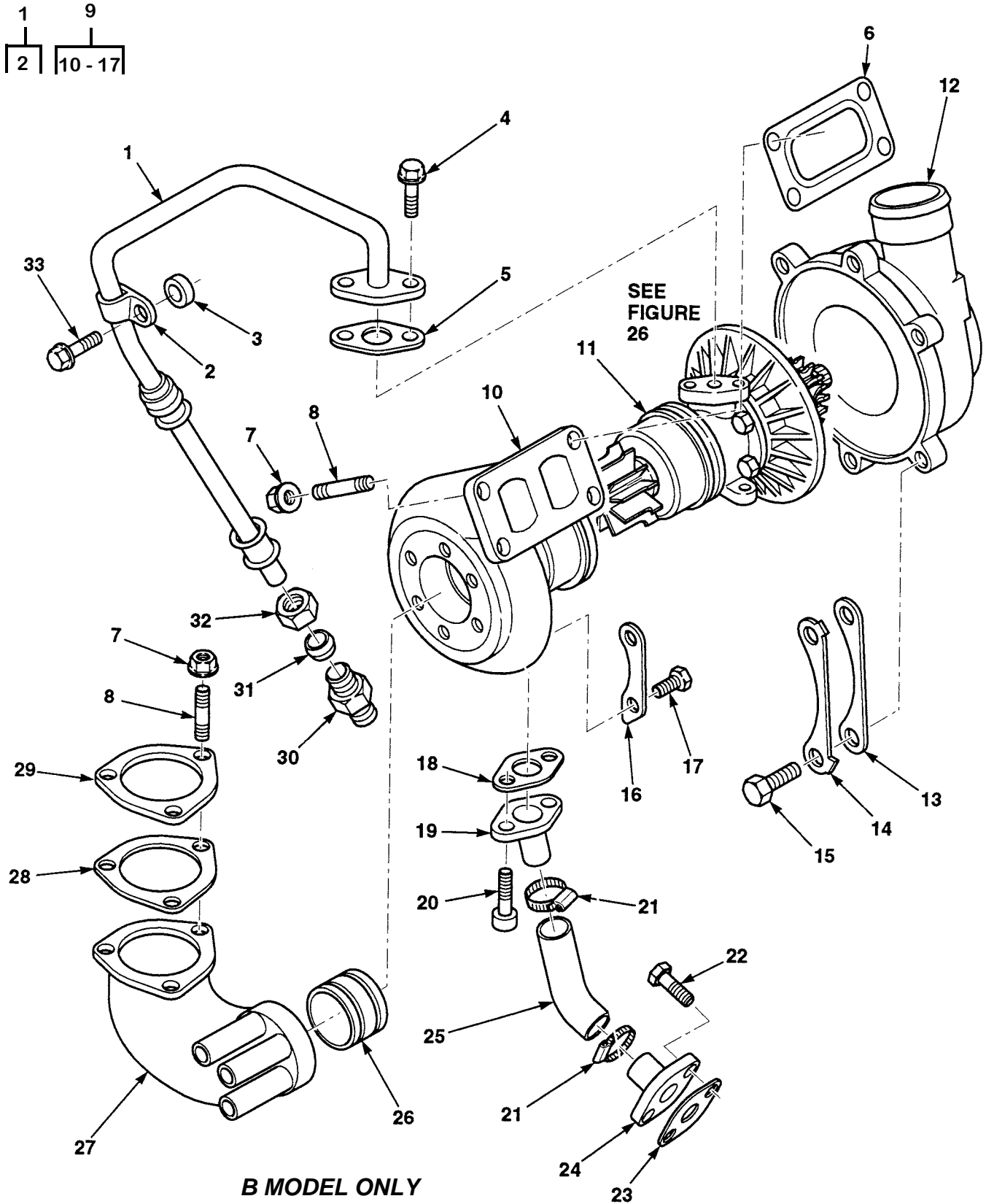
Figure 25. Turbocharger Assembly (Sheet 1 of 2)
