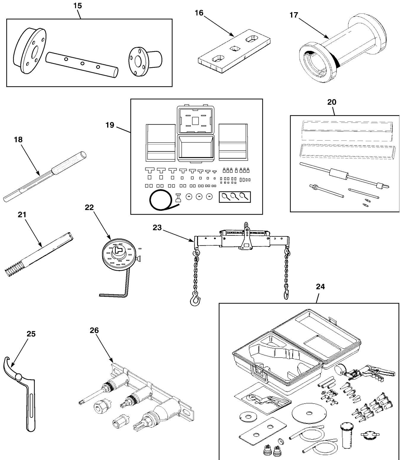
Figure 143. Direct Support Maintenance Special Tools (Sheet 2 of 2)
