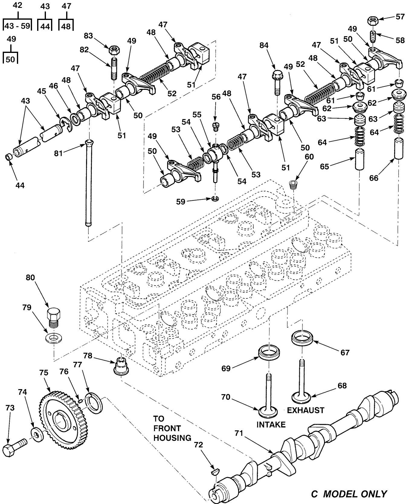
Figure 9. Valve, Rocker Arms, Pushrods, and Camshaft (Sheet 2 of 2)
