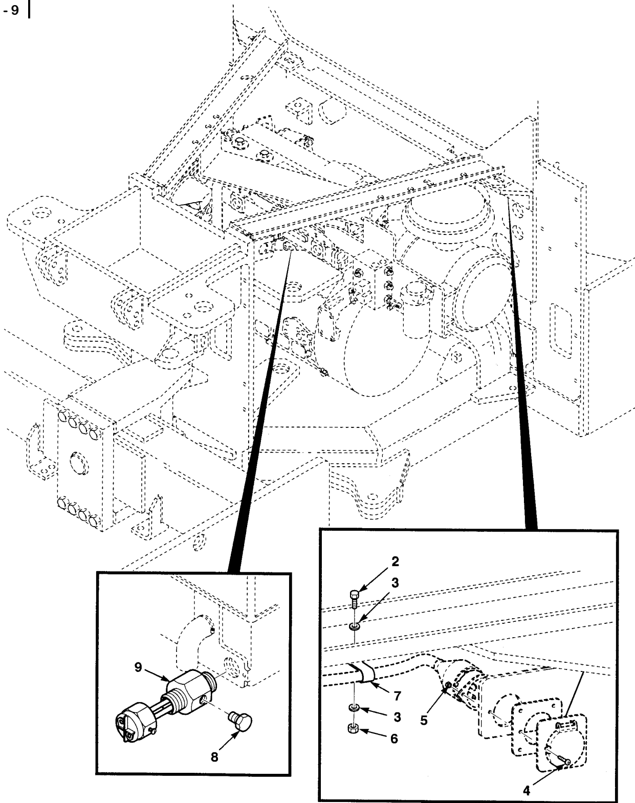
Figure 110. Engine Block Heating Element
