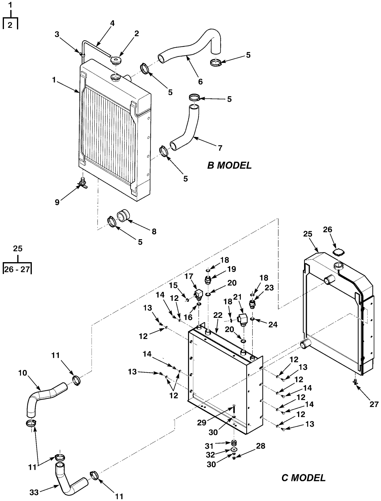
Figure 37. Radiator and Hoses
