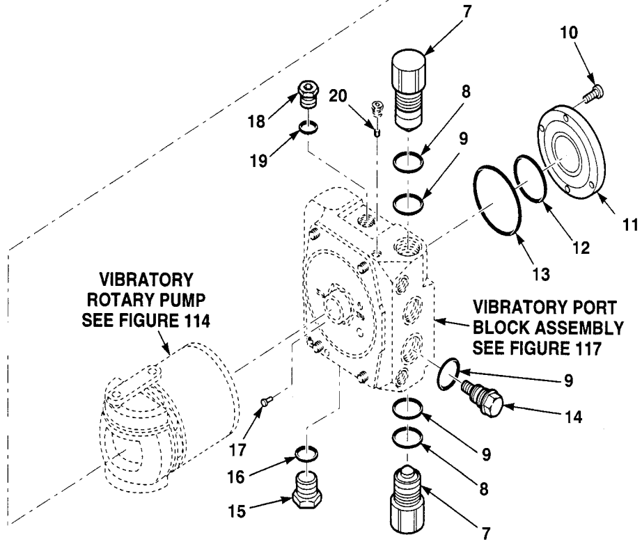
Figure 112. Vibratory Pump Assembly (Sheet 1 of 2)
