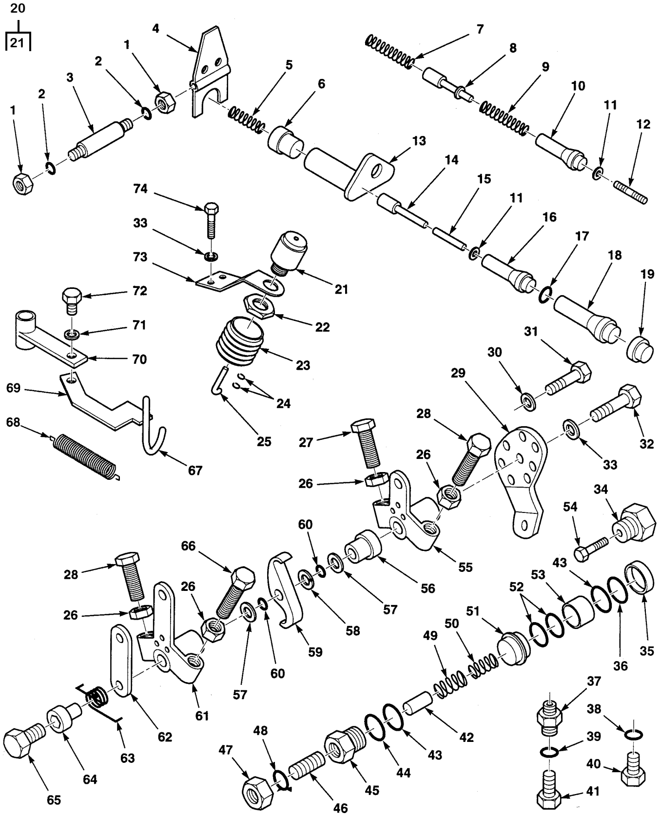
Figure 22. Fuel Injector Pump (External), B Model Only
