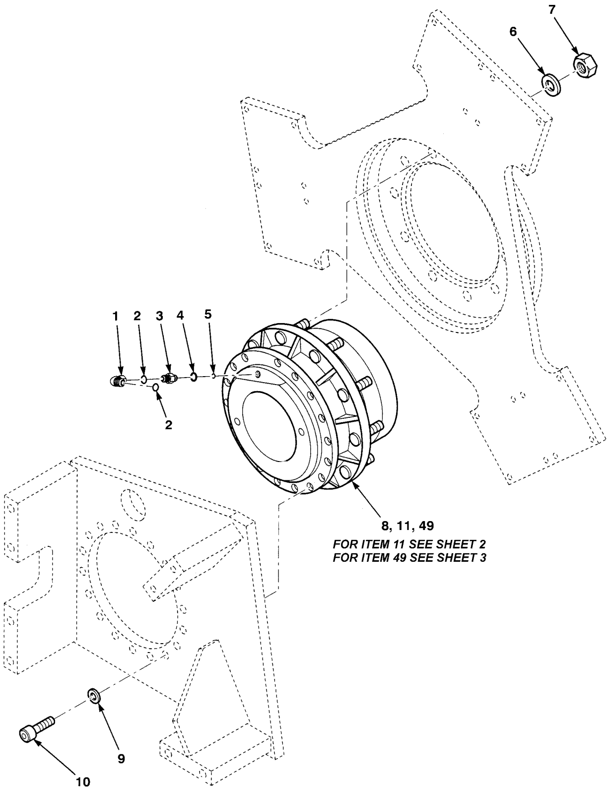
Figure 80. Front Propeller Gearbox Assembly (Sheet 1 of 3)
