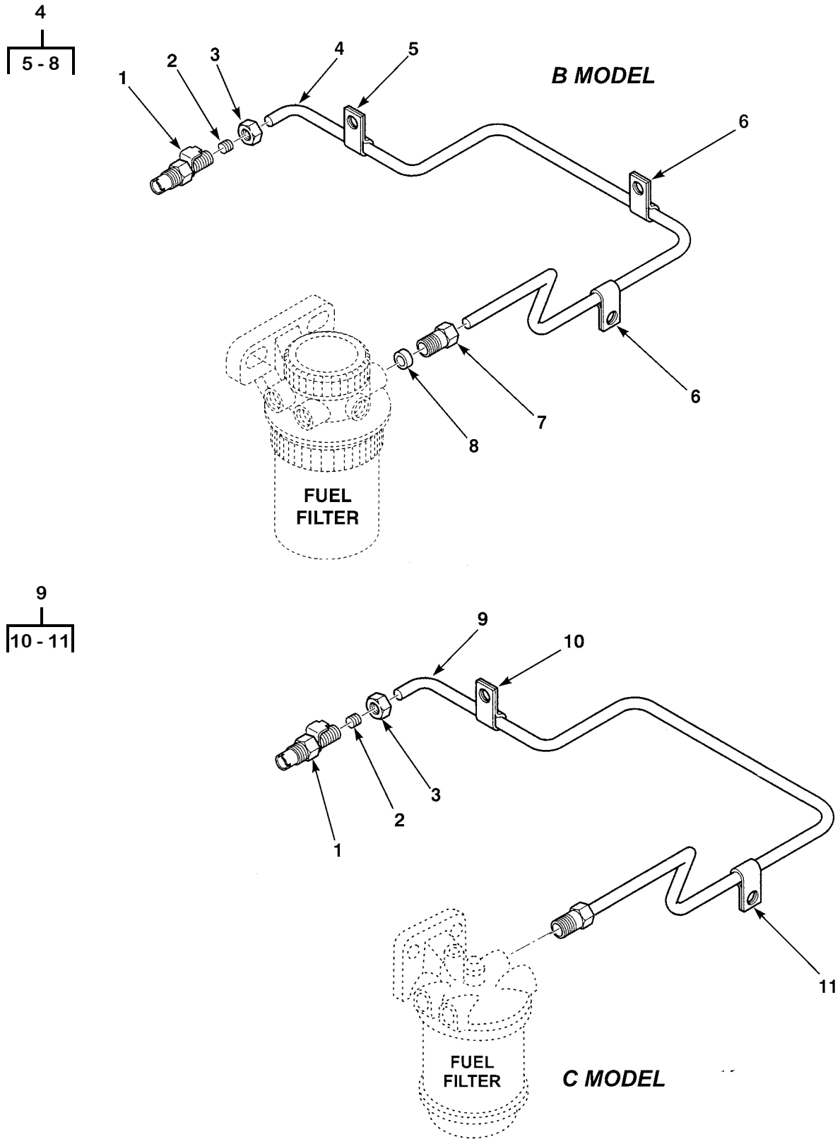
Figure 34. Cold Start Heater
