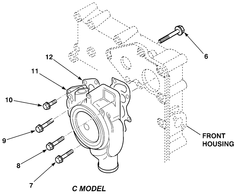
Figure 40. Engine Water Pump
