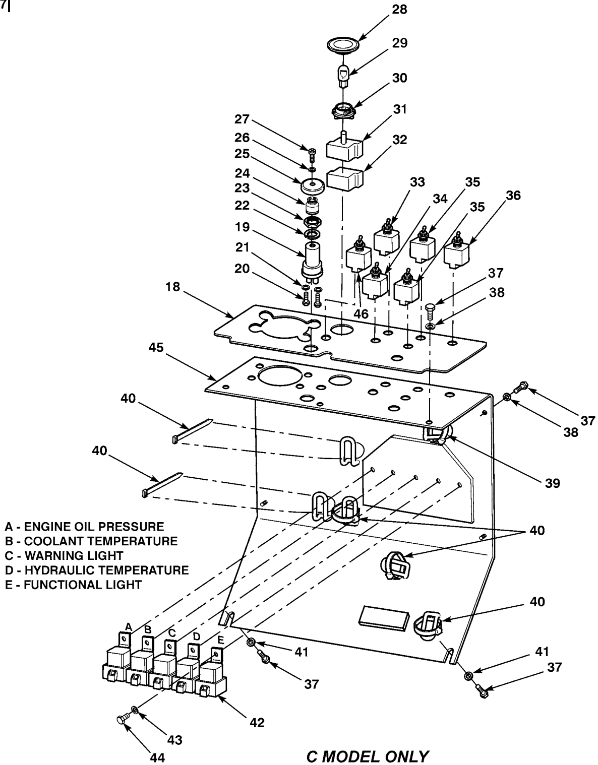
Figure 49. Switches (Sheet 2 of 2)
