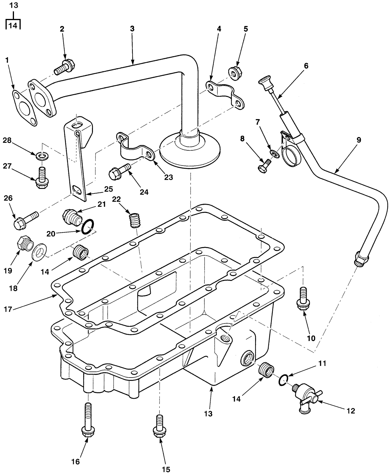
Figure 14. Oil Pan and Oil Level Gage
