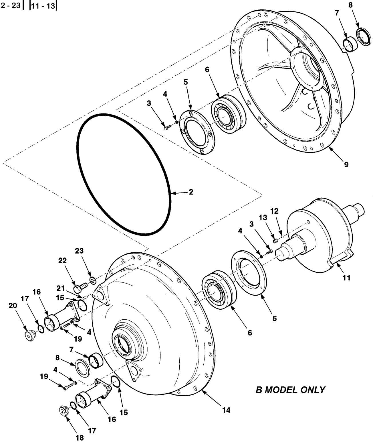
Figure 131. Front and Rear Eccentric Weight and Shaft (Sheet 1 of 2)
