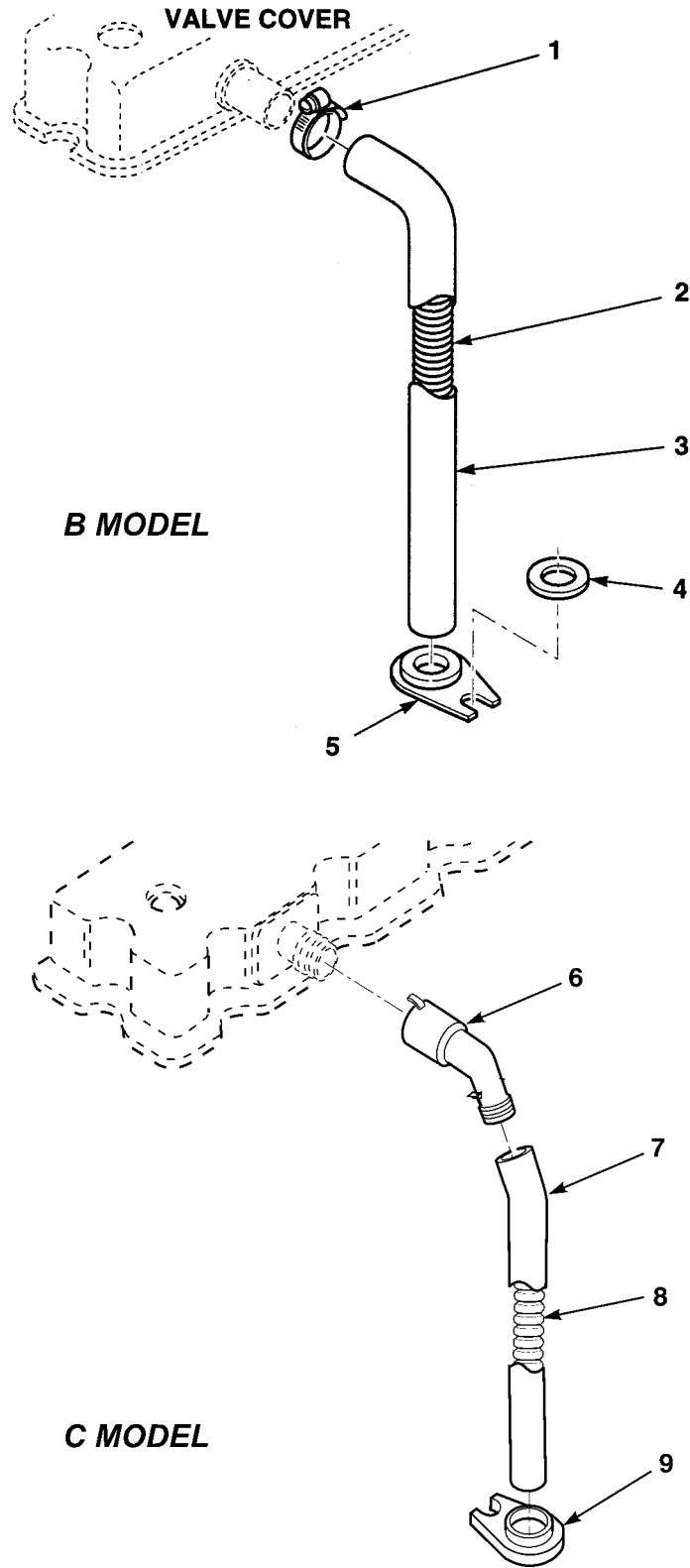
Figure 12. Breather Tube
