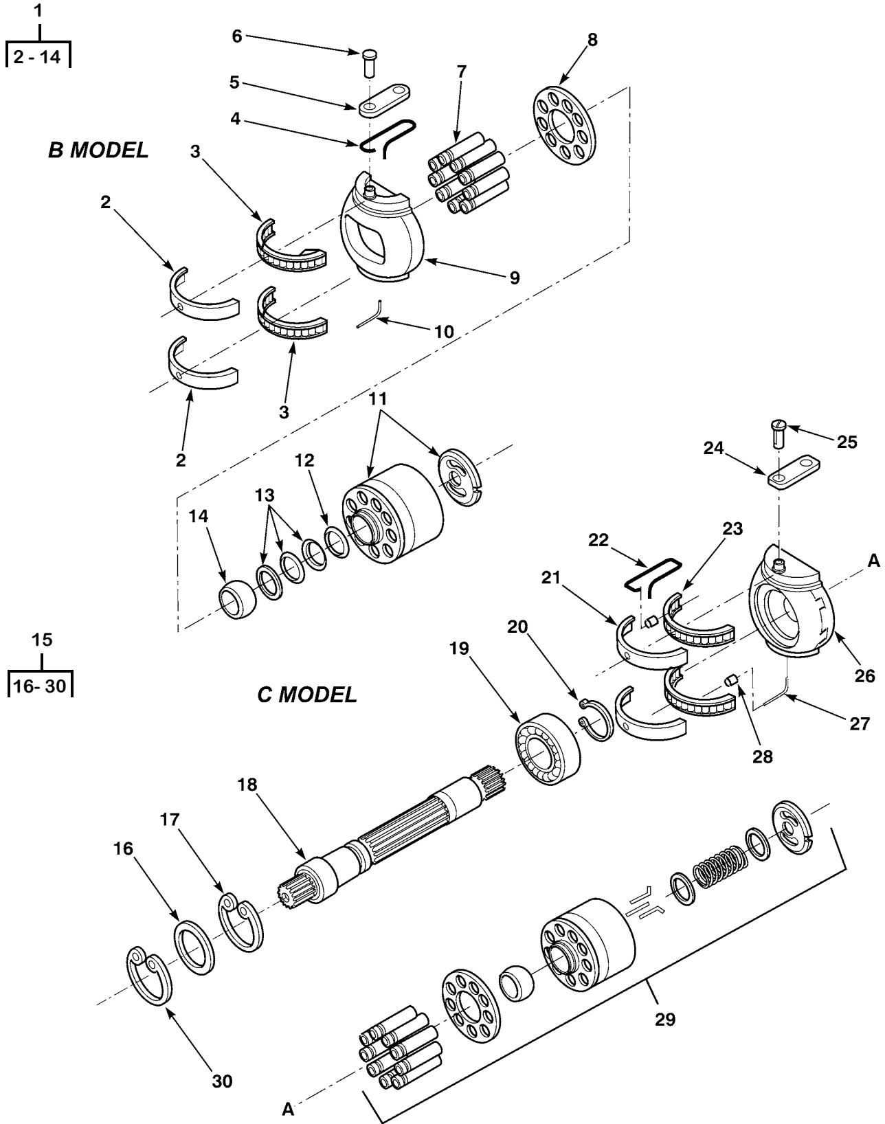
Figure 114. Vibratory Rotary Pump
