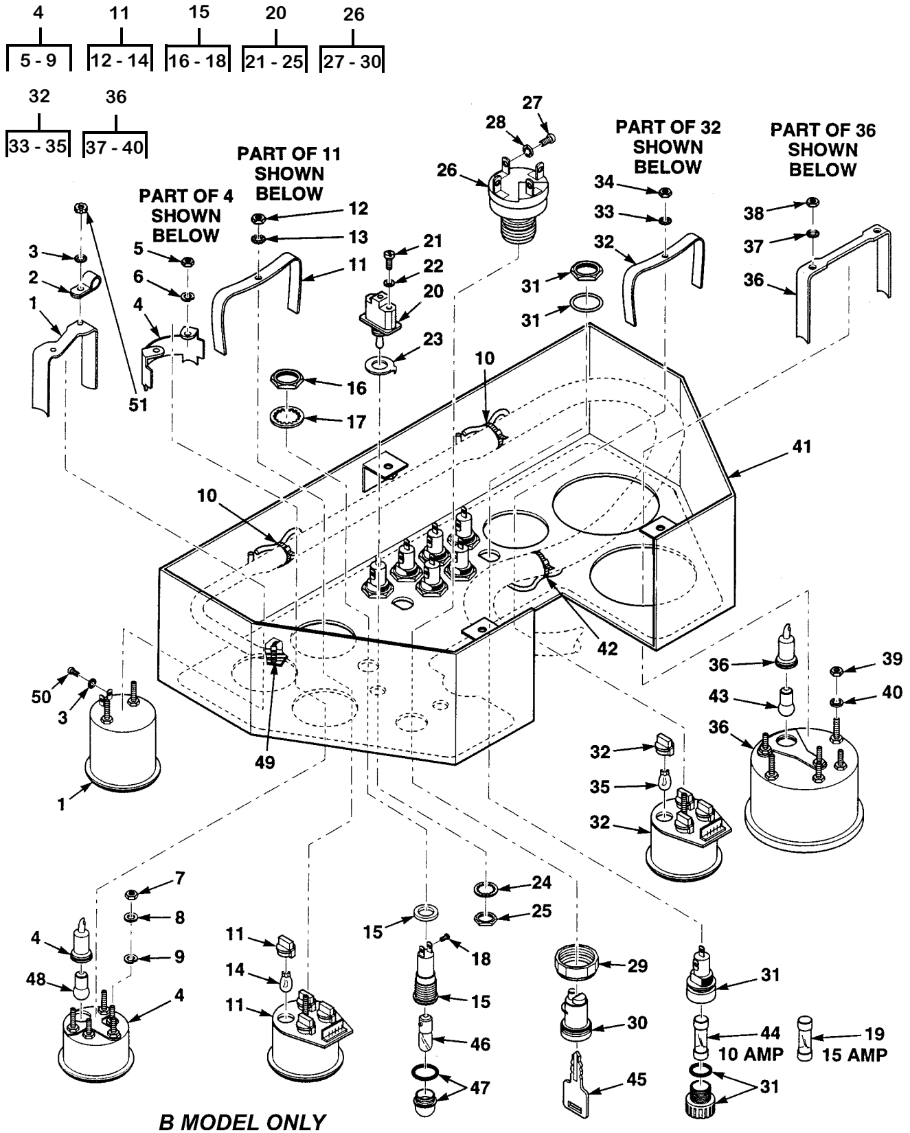
Figure 48. Instrument Panel and Gages (Sheet 1 of 2)
