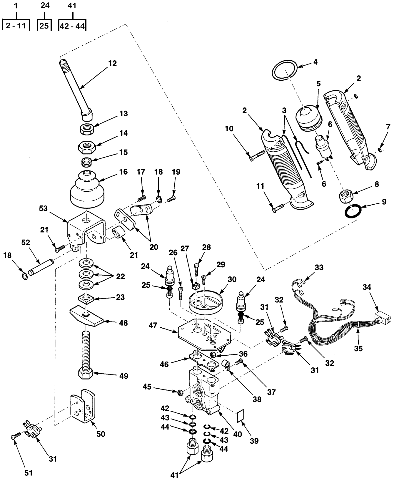
Figure 78. Propeller Control Valve and Lever Assembly
