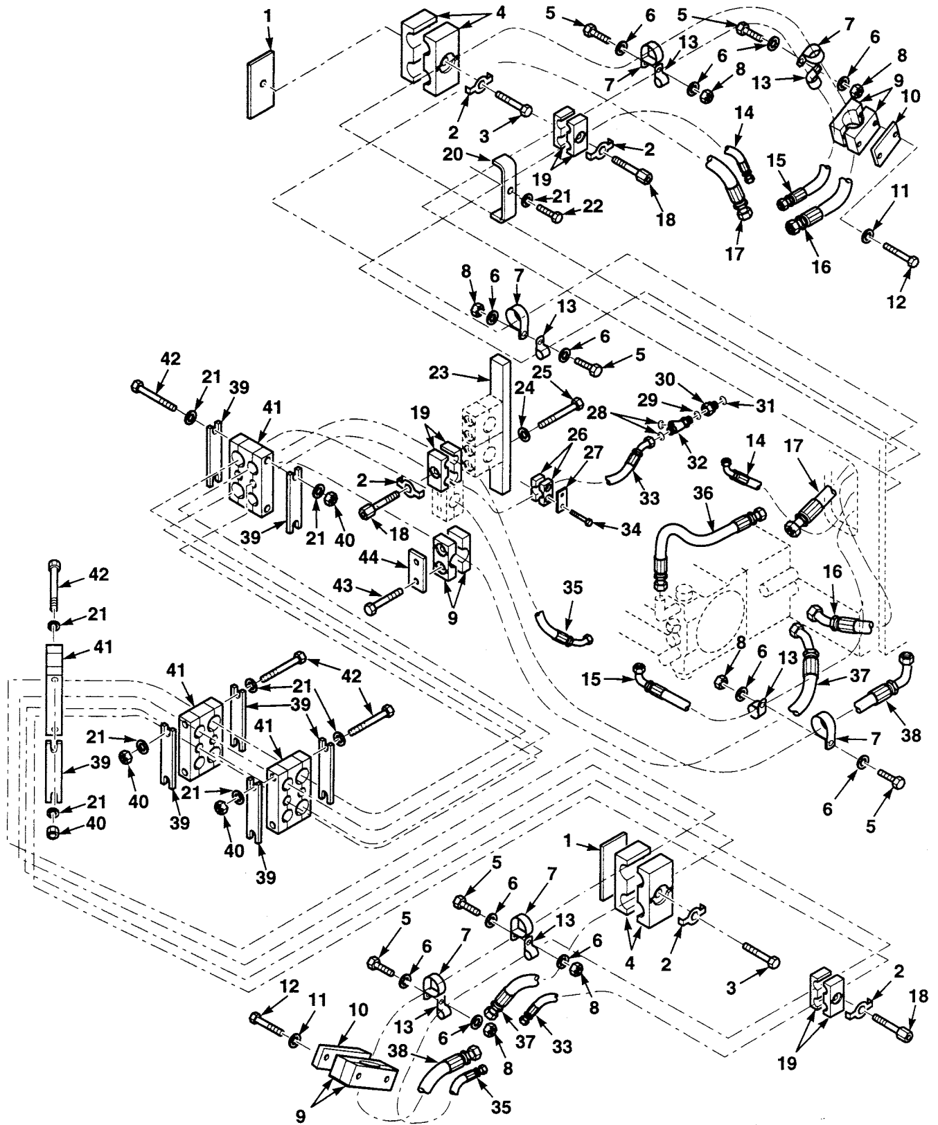
Figure 128. Vibratory Lines and Fittings
