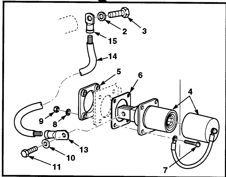
Figure 54. Batteries and NATO Connector
