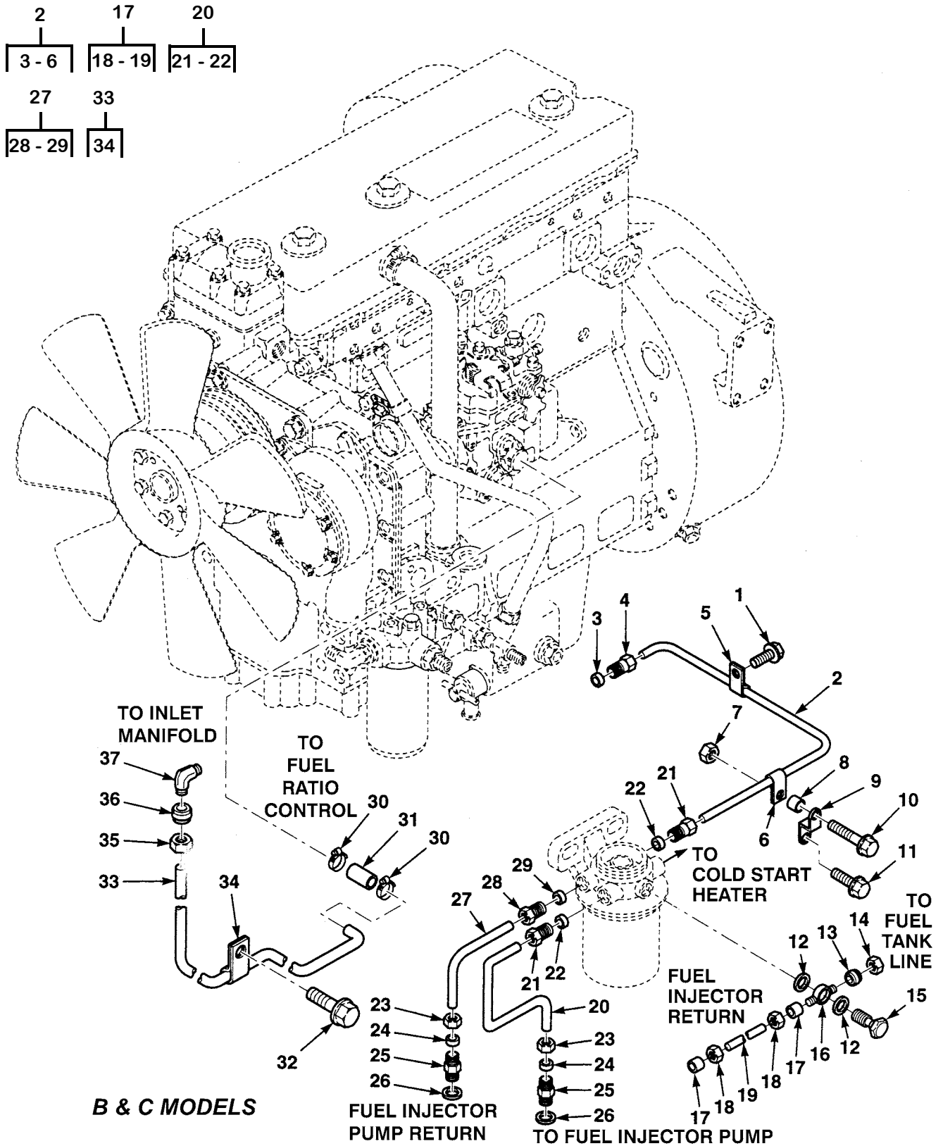
Figure 18. Engine Fuel Lines and Fittings
