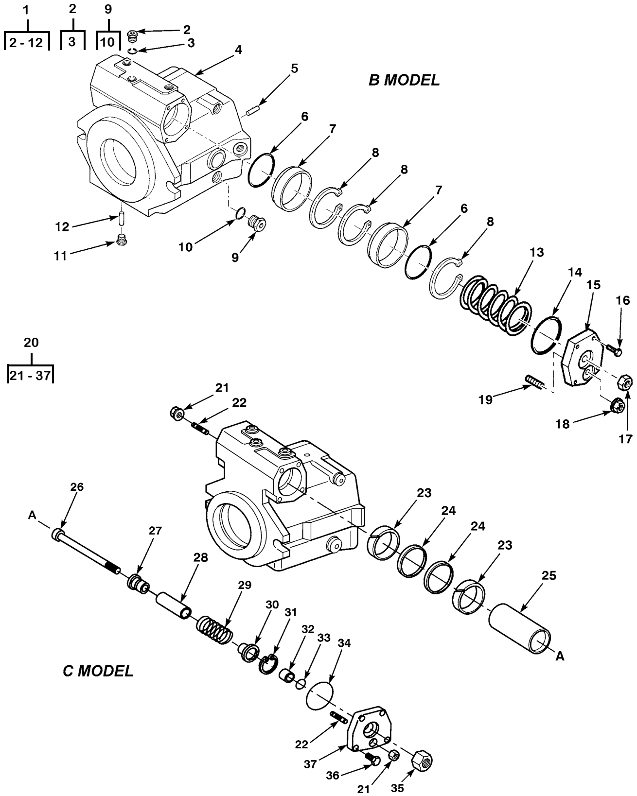
Figure 115. Vibratory Housing Assembly
