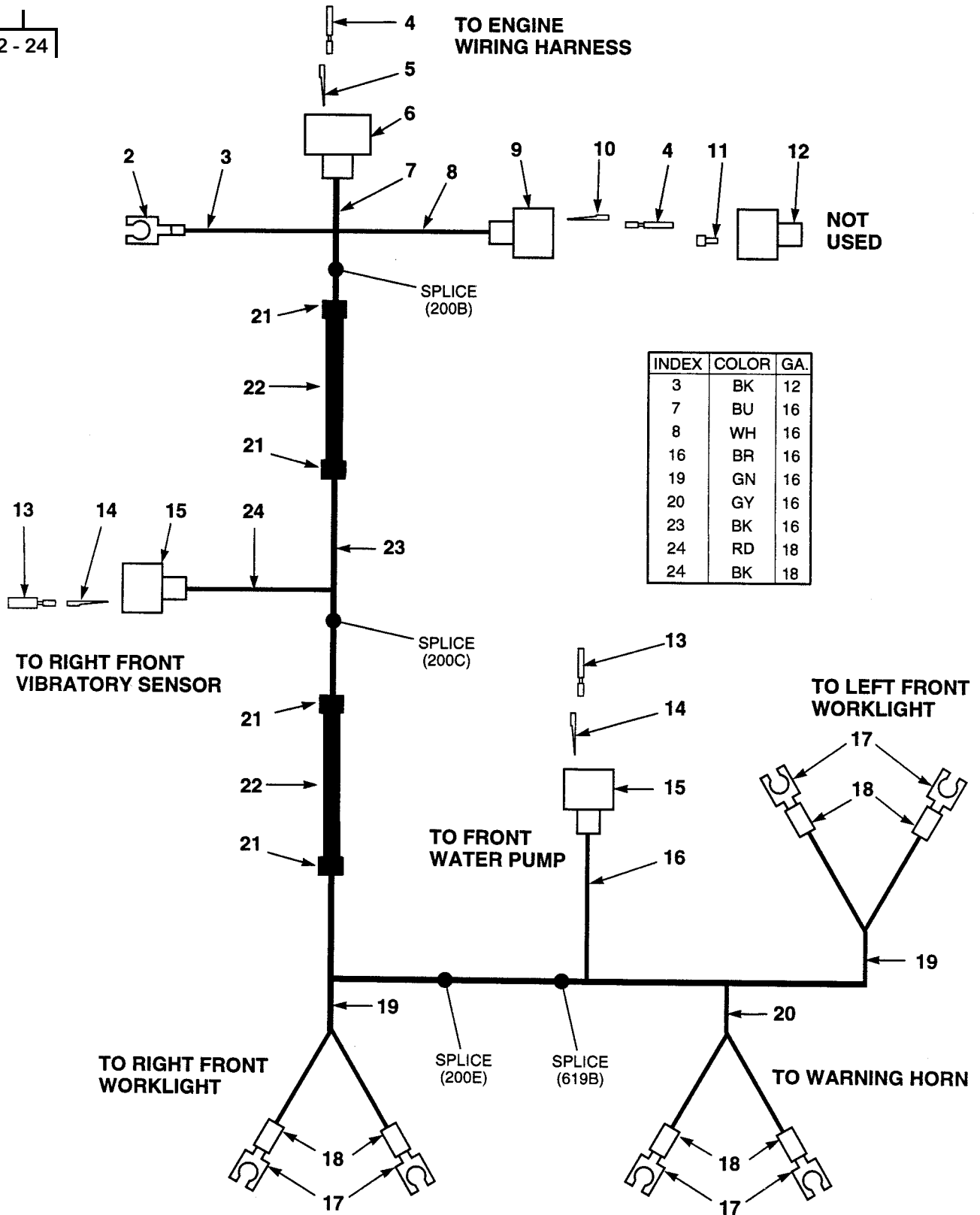
Figure 59. Front Wiring Harness
