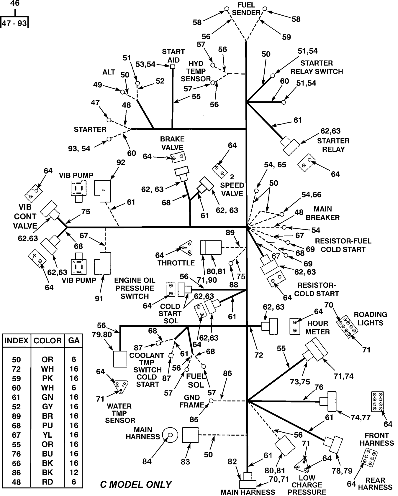
Figure 57. Engine Wiring Harness (Sheet 2 of 2)
