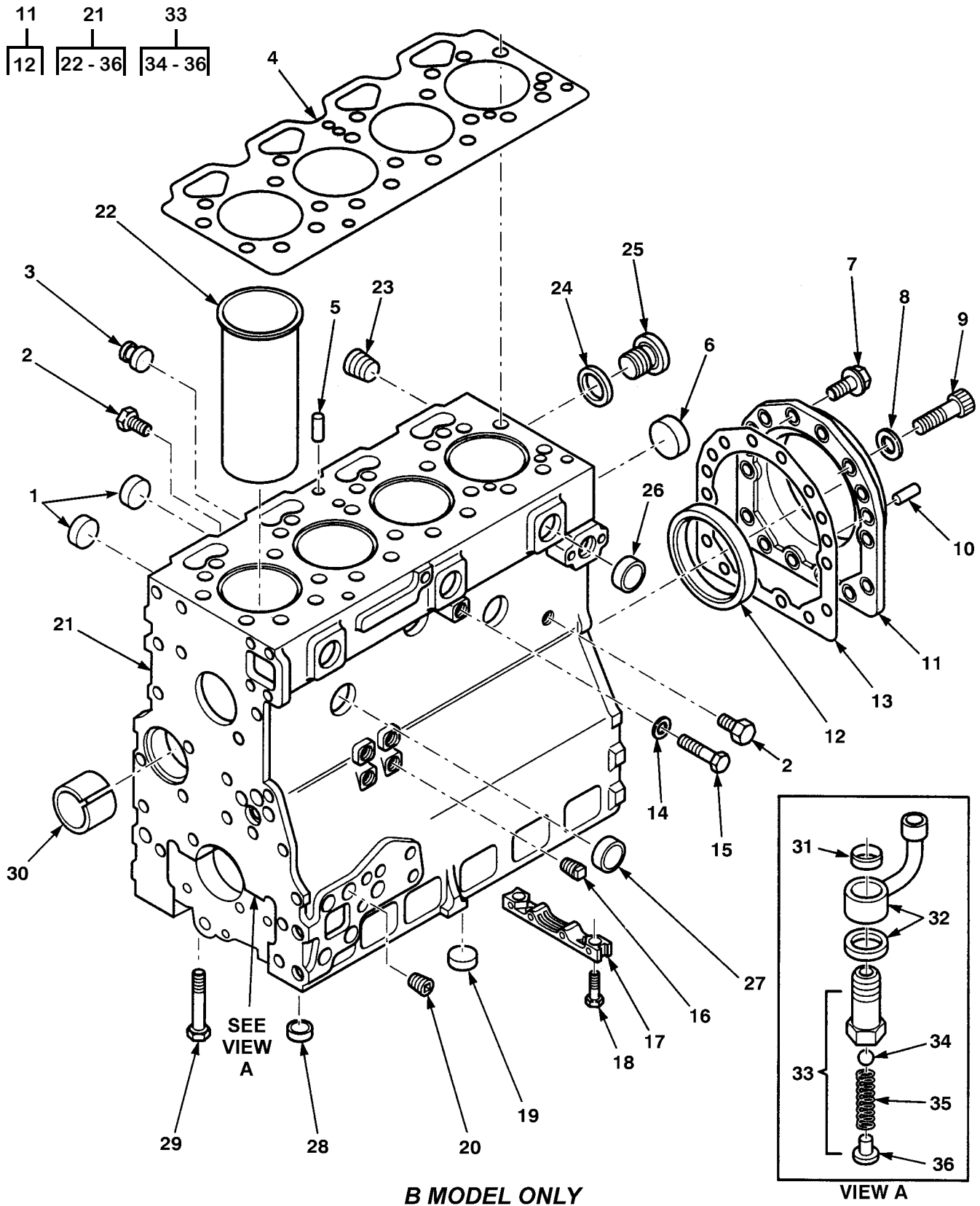
Figure 2. Cylinder Block Assembly (Sheet 1 of 2)
