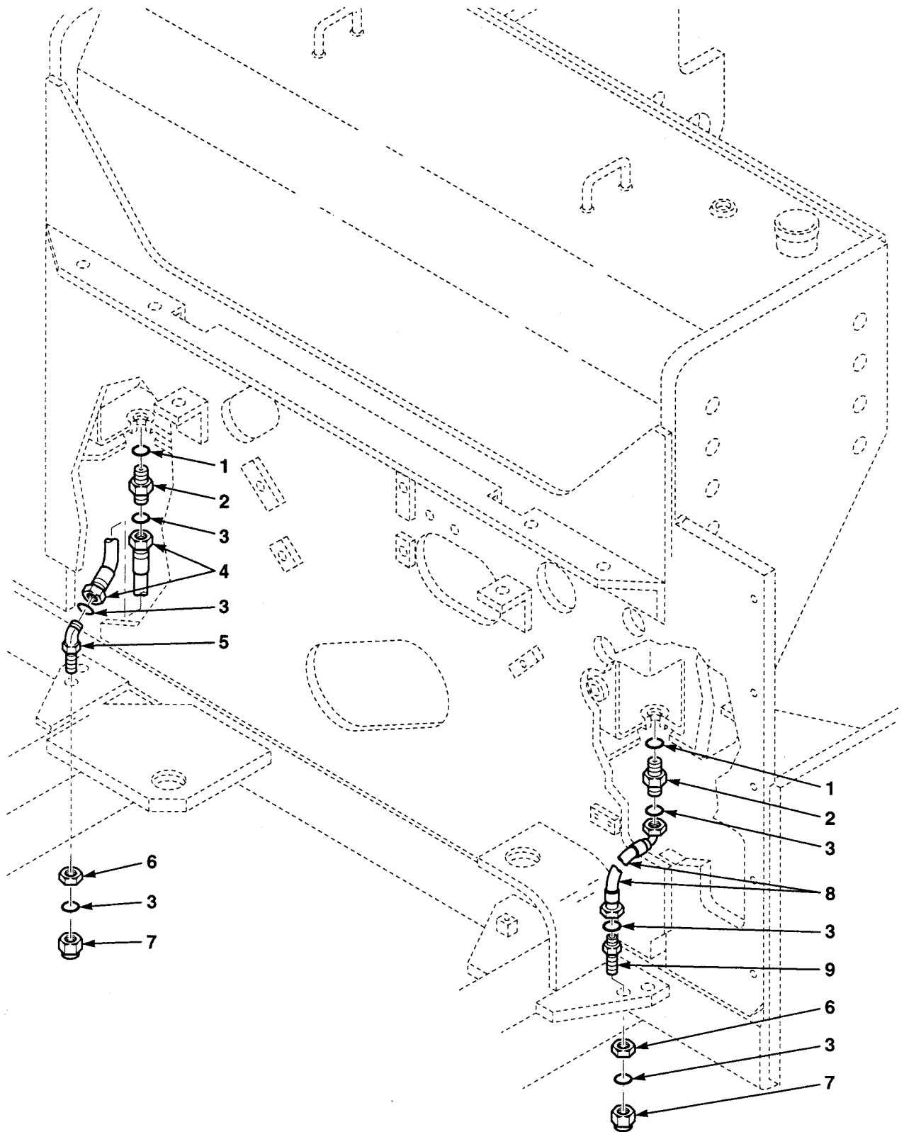
Figure 28. Fuel/Hydraulic Oil Tank Drain Lines
