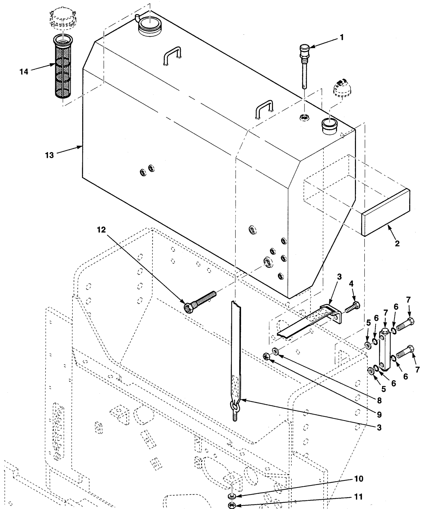
Figure 29. Fuel/Hydraulic Oil Tank and Mounting Hardware
