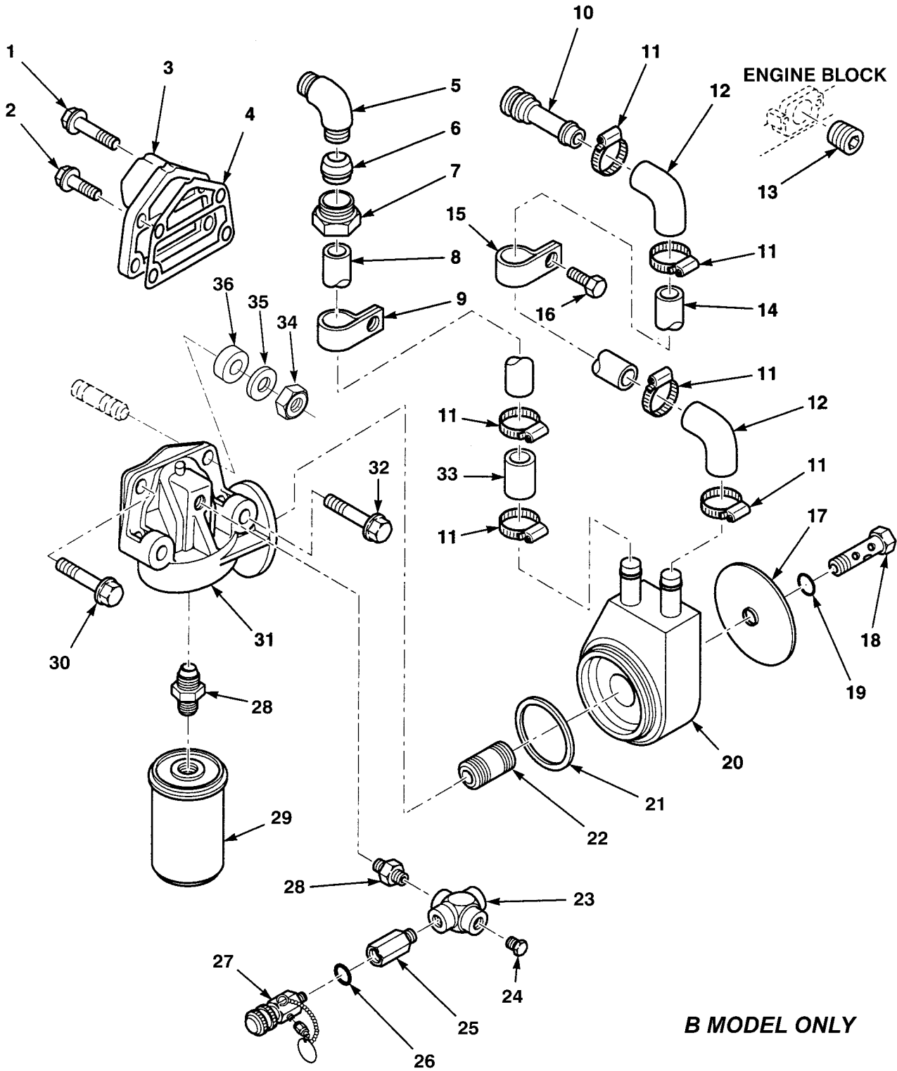
Figure 15. Engine Oil Filter and Cooler Assembly (Sheet 1 of 2)
