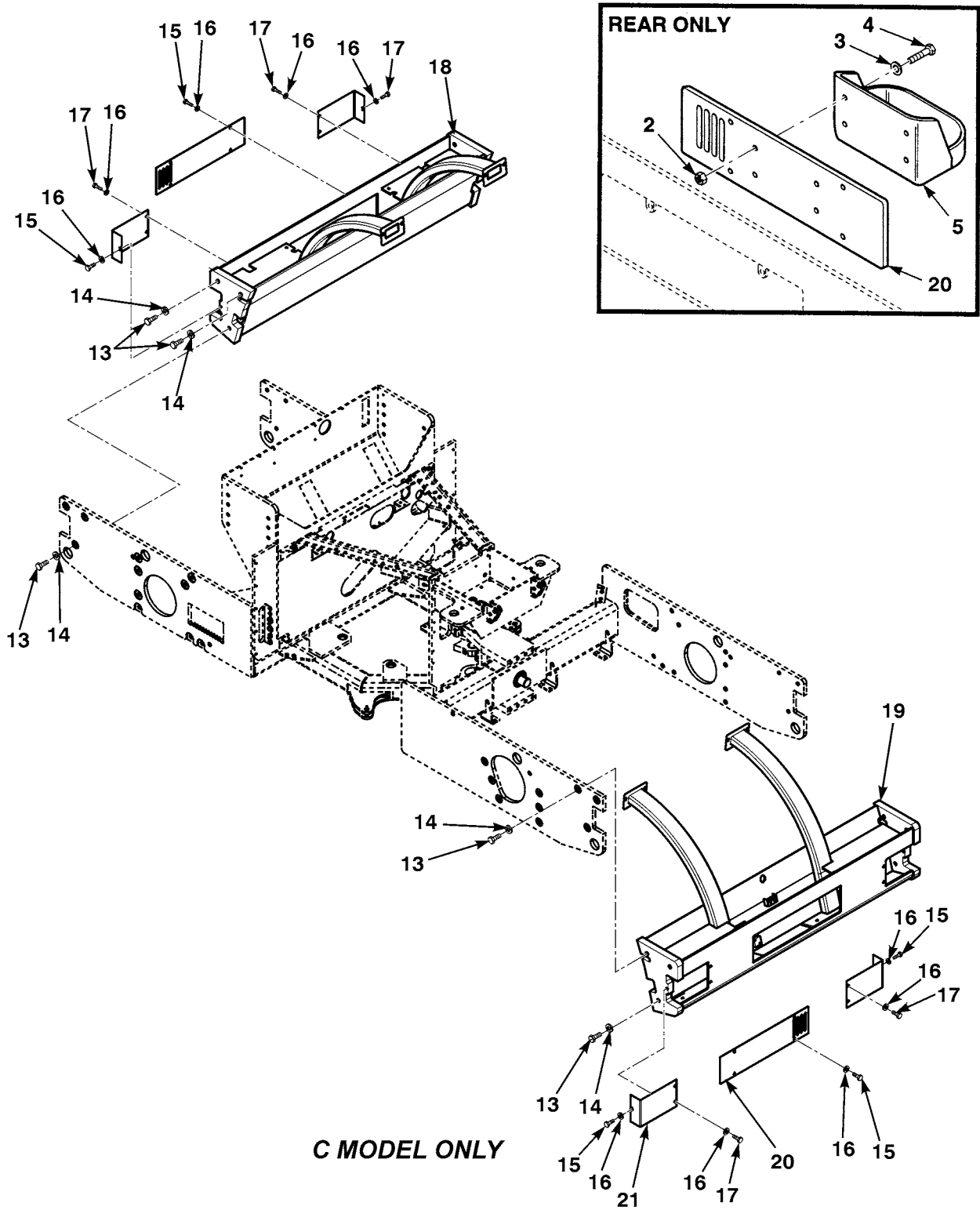
Figure 96. Bumper Assemblies (Sheet 2 of 2)
