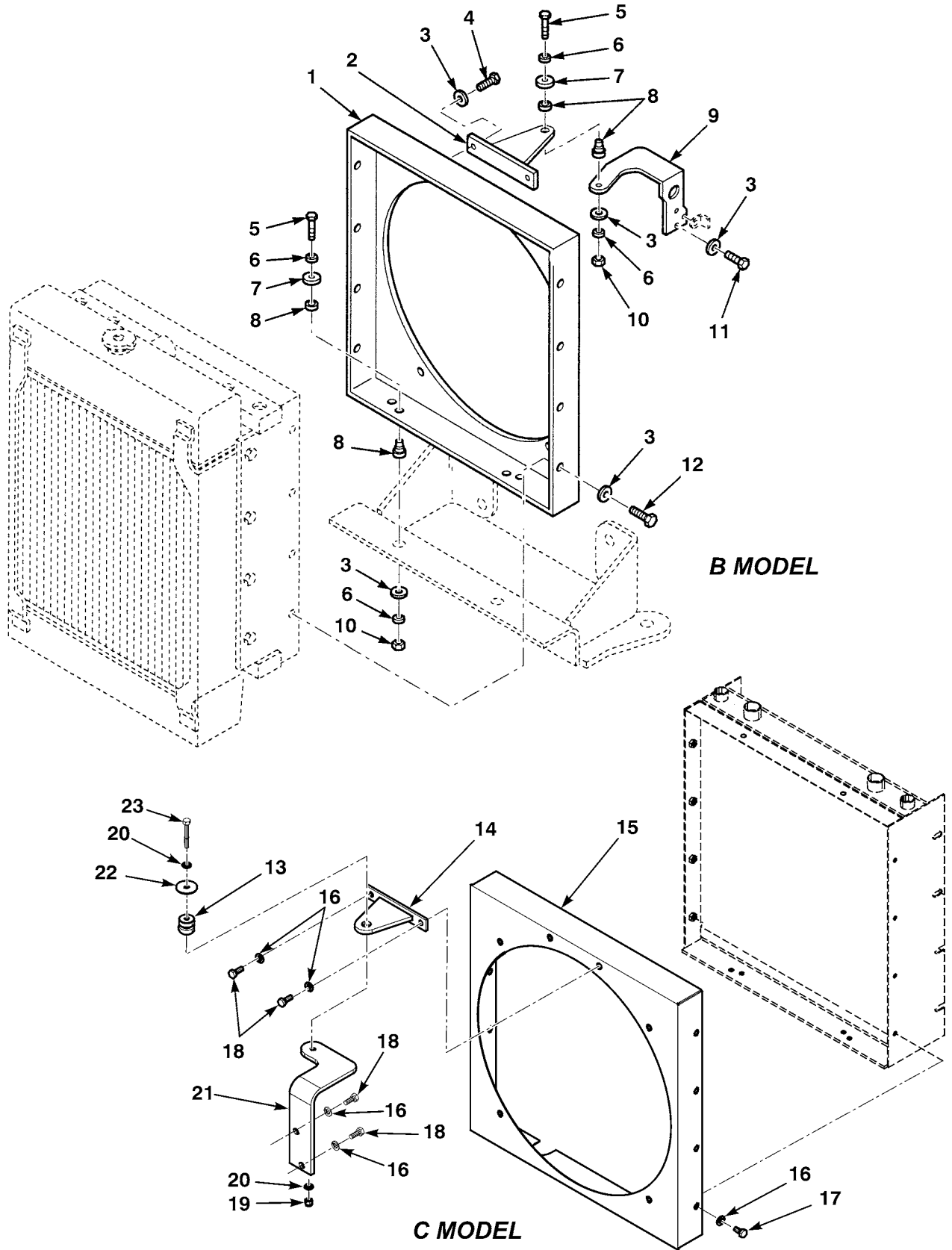
Figure 38. Fan Shroud
