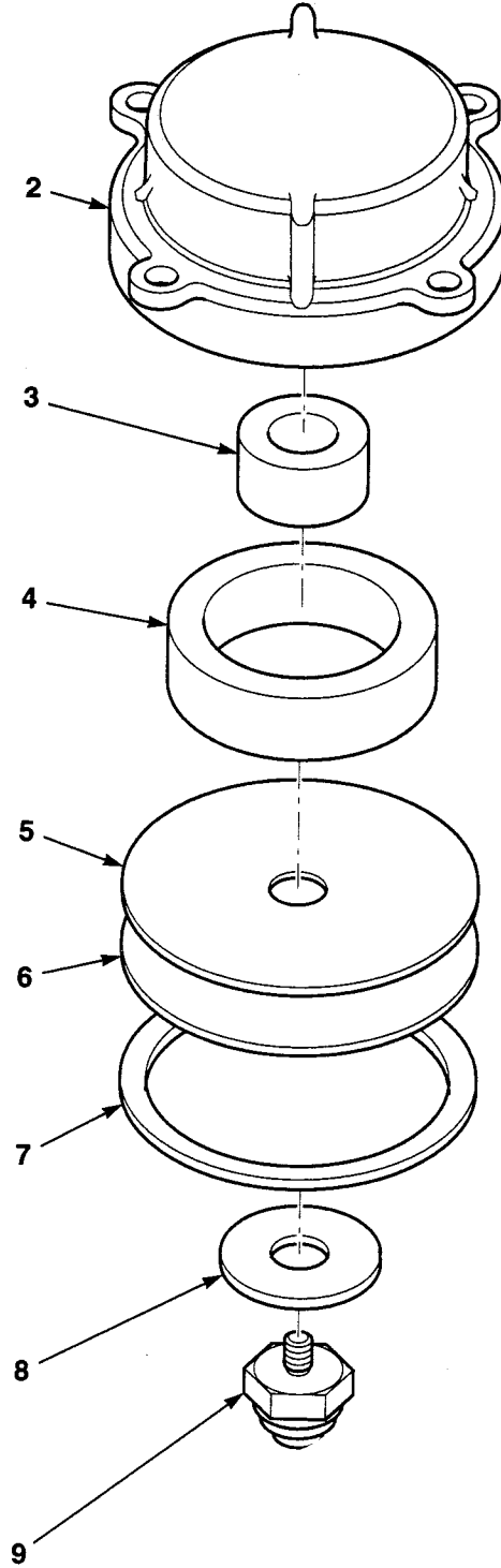
Figure 30. Fuel Cap Assembly
