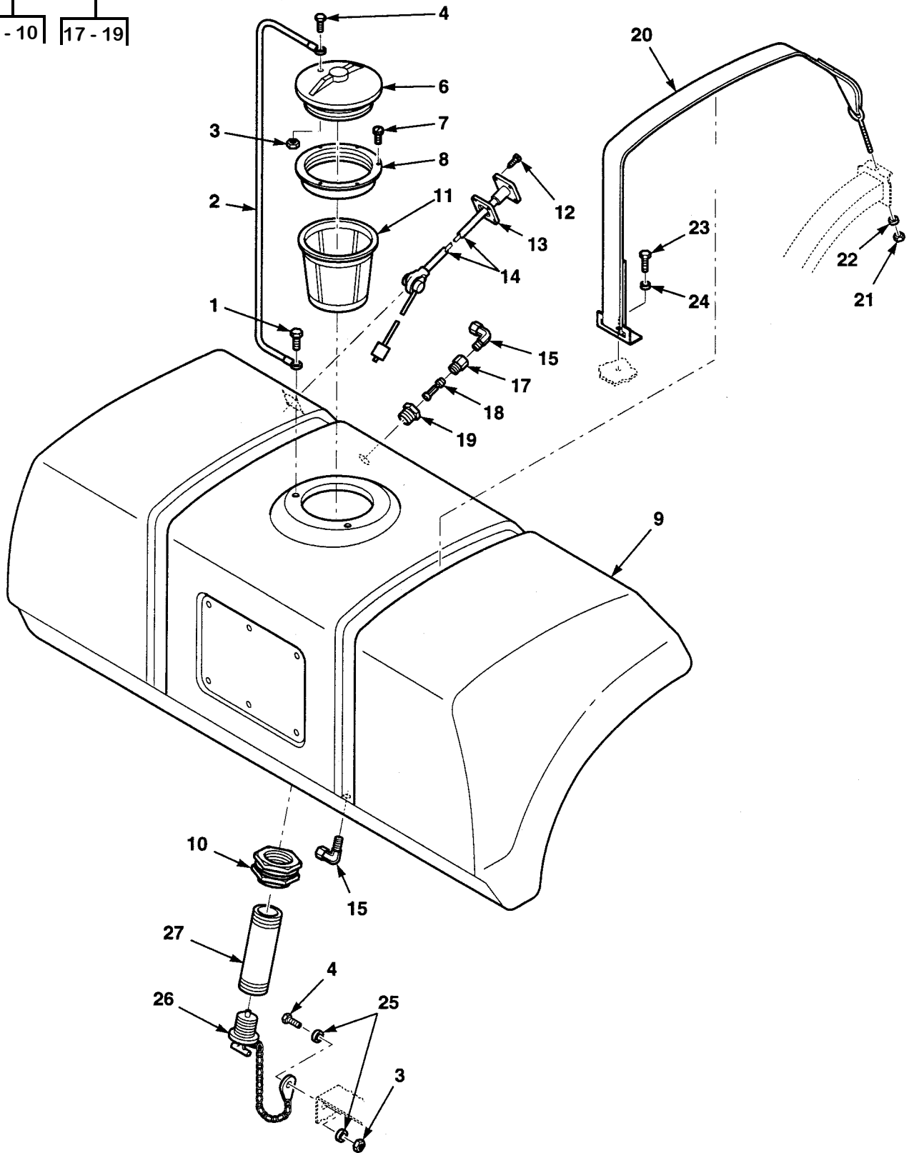
Figure 134. Front and Rear Water Tanks and Strainer
