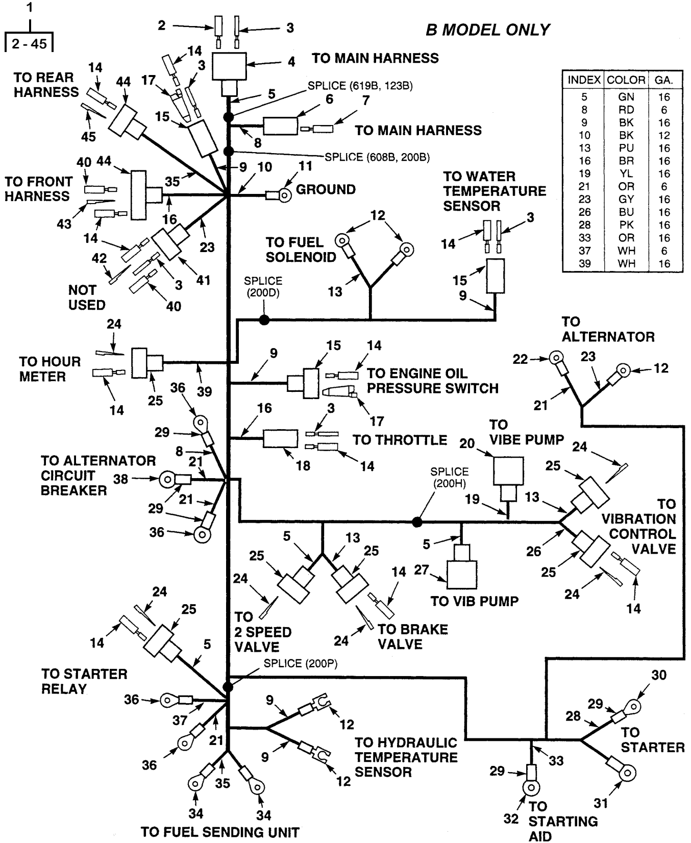
Figure 57. Engine Wiring Harness (Sheet 1 of 2)
