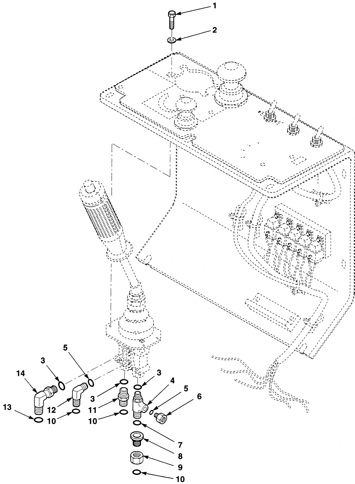
Figure 77. Propeller Control Valve Fittings
