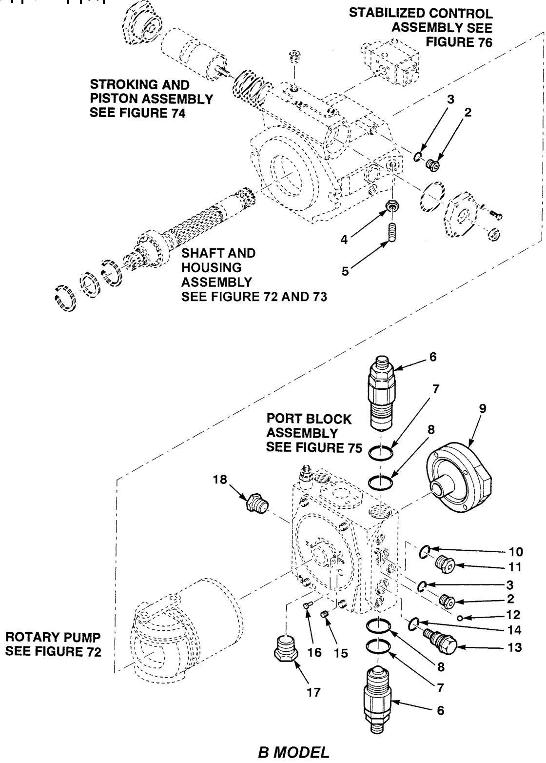
Figure 71. Hydraulic Propel Pump (Sheet 1 of 2)
