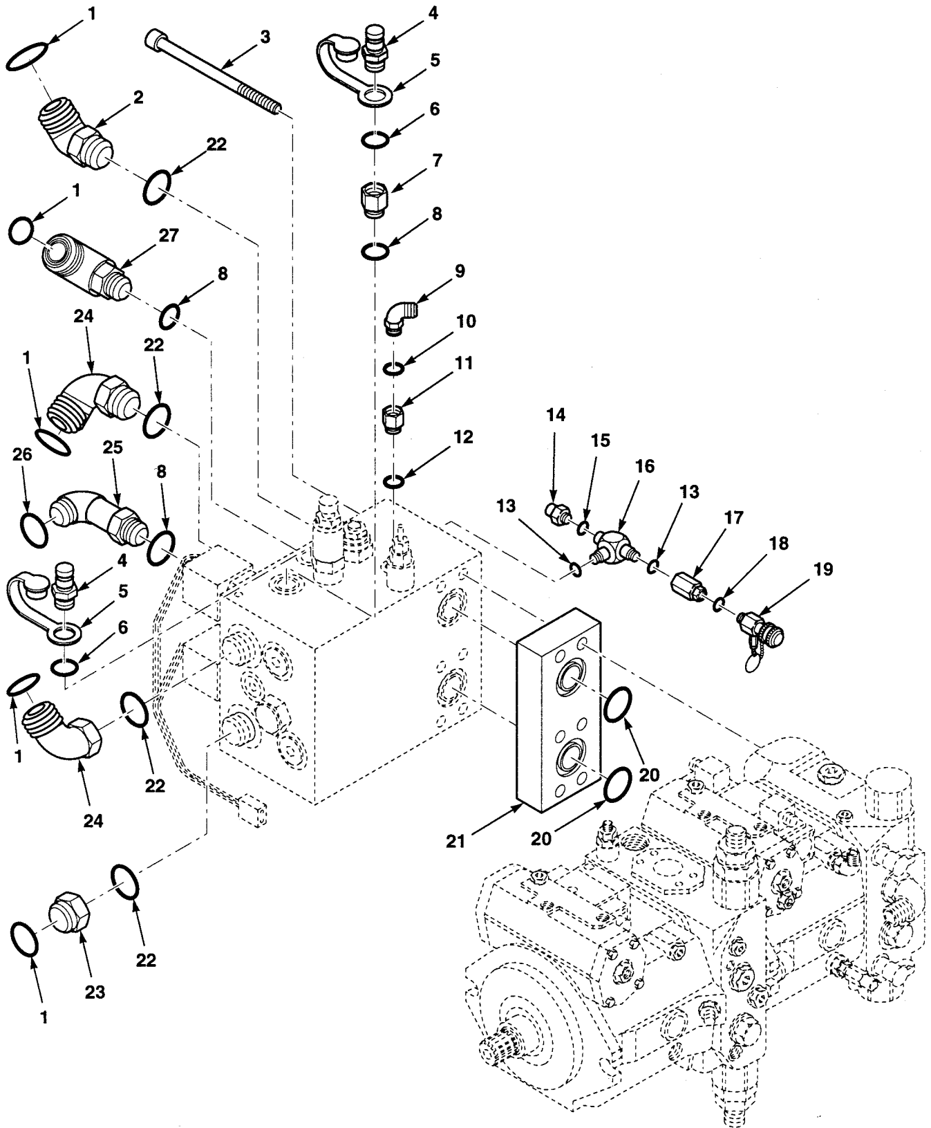
Figure 122. Vibratory Cooling Control Valve Fittings
