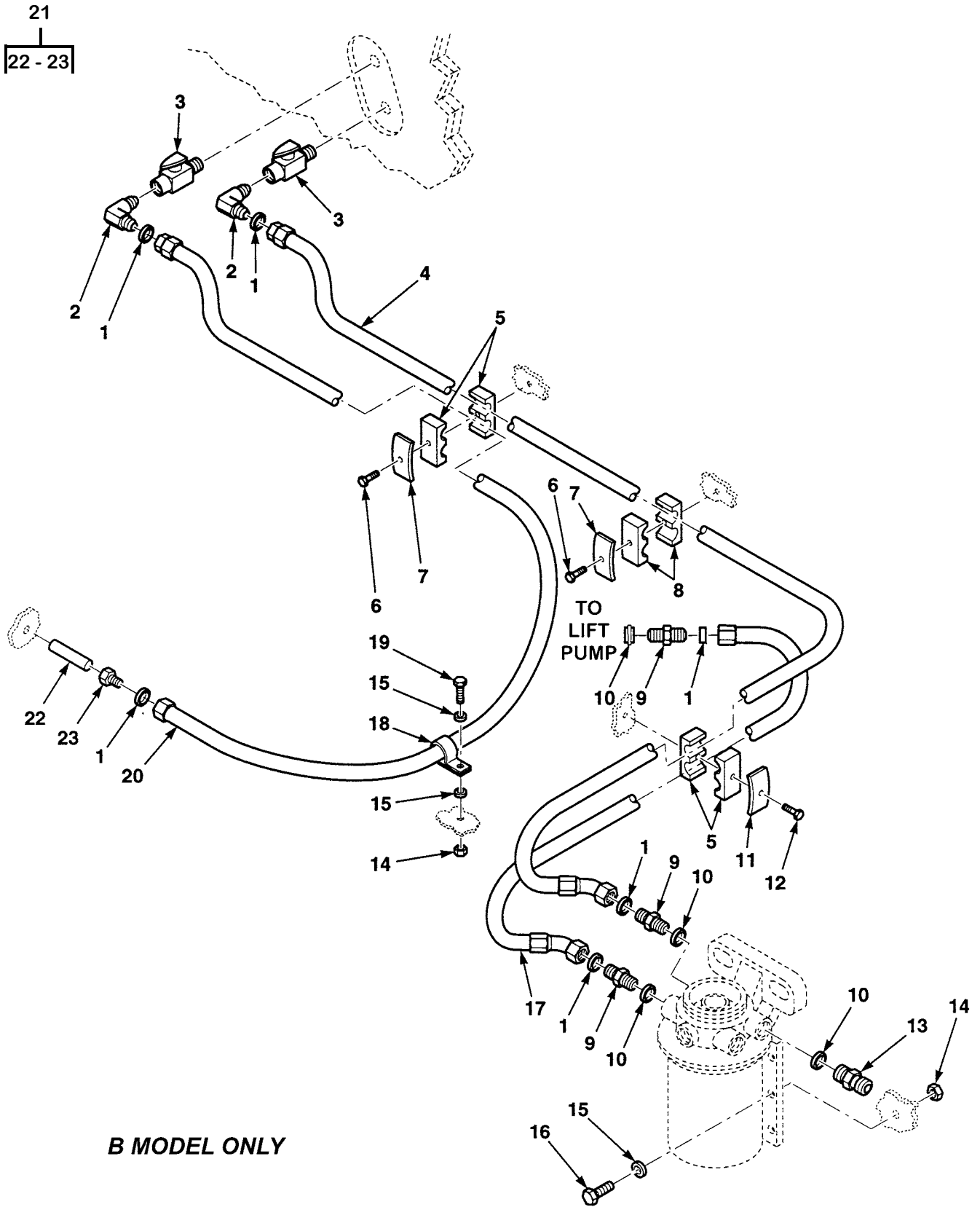
Figure 27. Fuel Lines and Fittings (Sheet 1 of 2)
