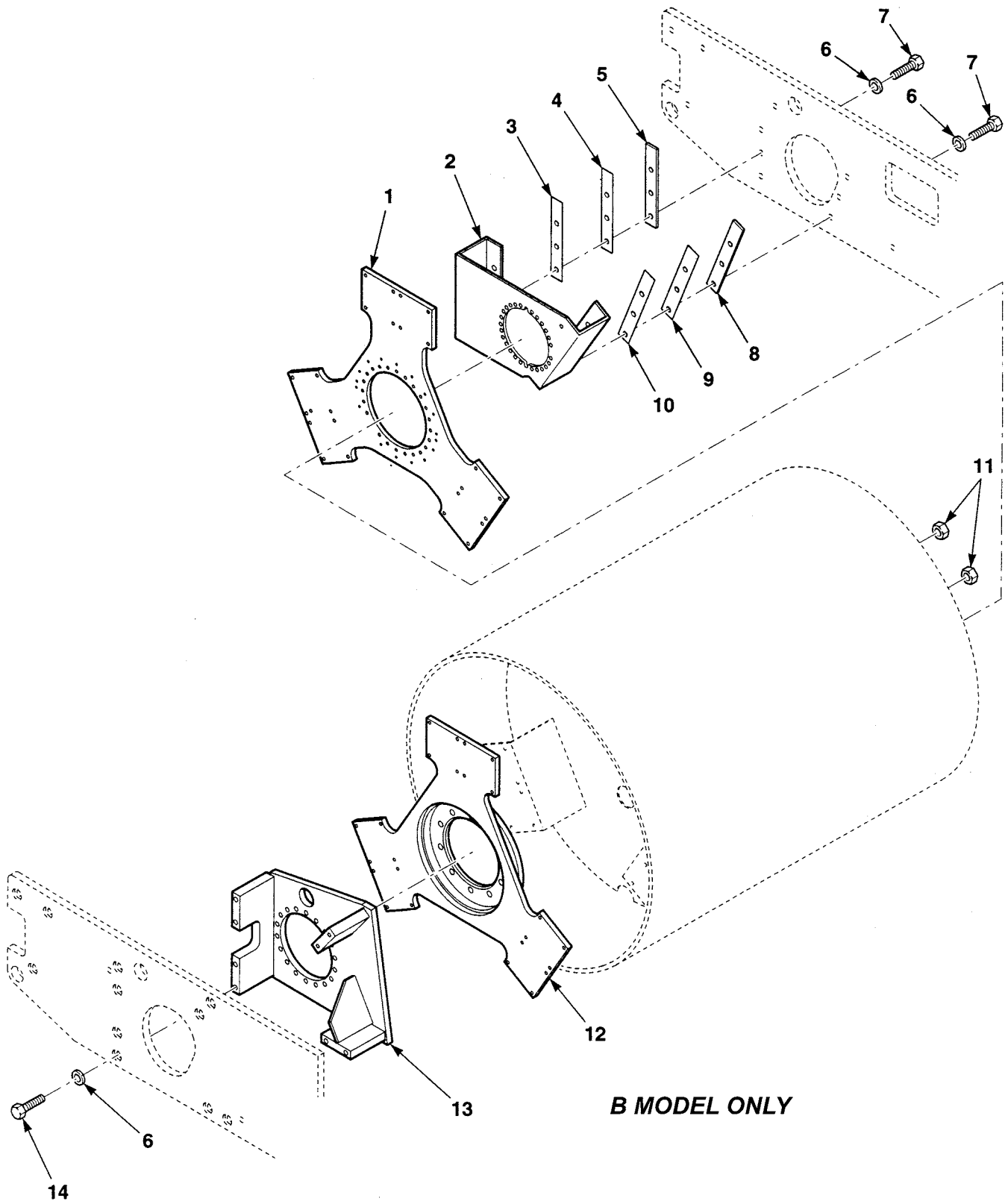
Figure 97. Front and Rear Drum Drive Mounting (Sheet 1 of 2)
