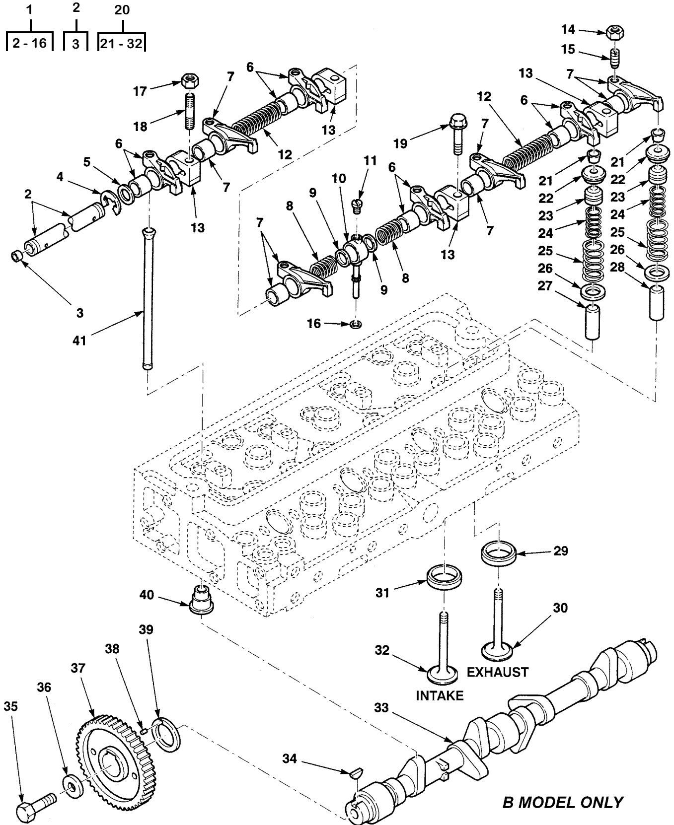
Figure 9. Valve, Rocker Arms, Pushrods, and Camshaft (Sheet 1 of 2)
