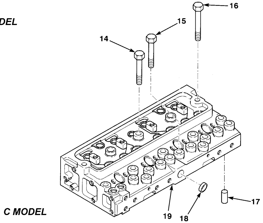
Figure 3. Cylinder Head Assembly
