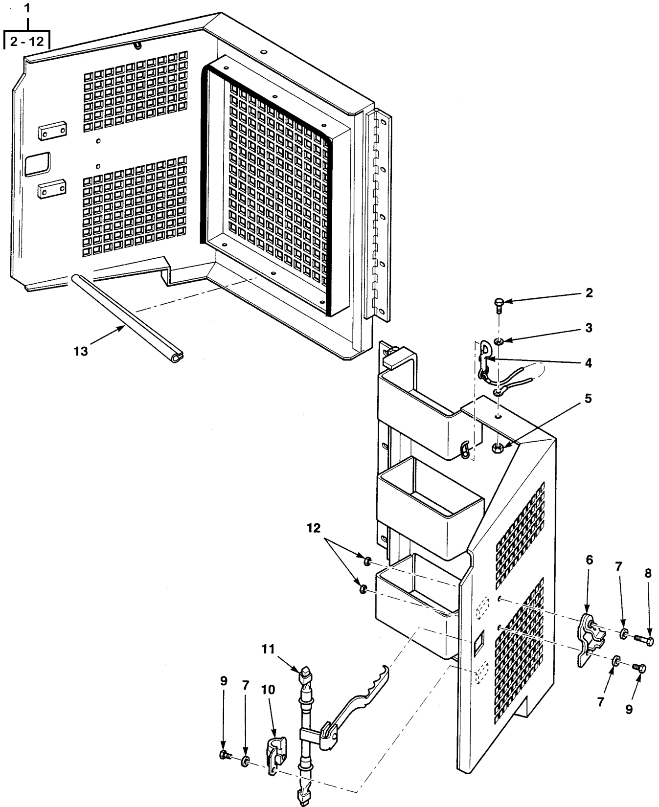
Figure 100. Door Assemblies
