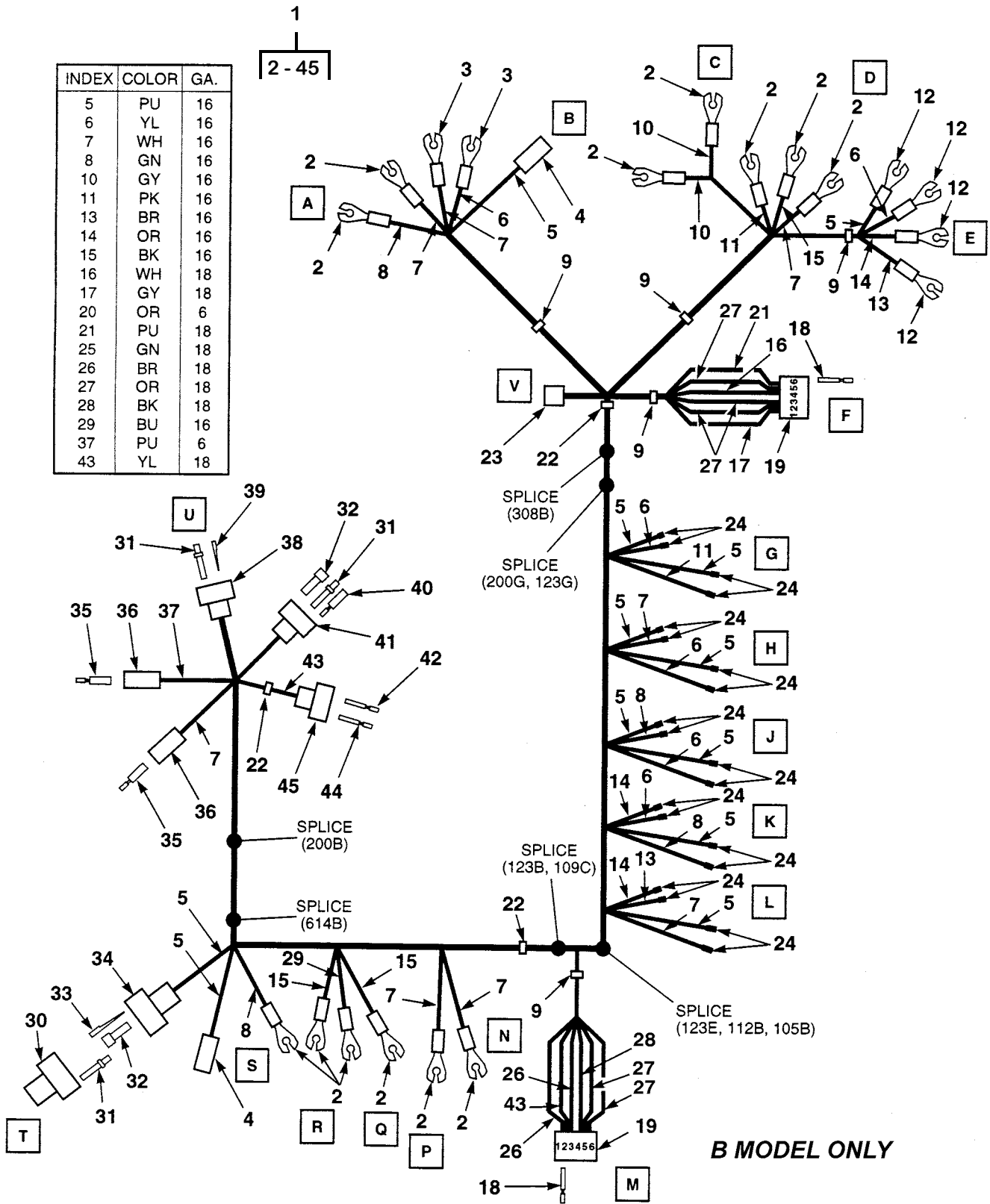
Figure 62. Instrument Harness Assembly (Sheet 1 of 3)
