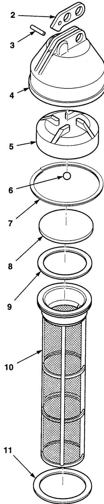
Figure 31. Hydraulic Oil Cap Assembly
