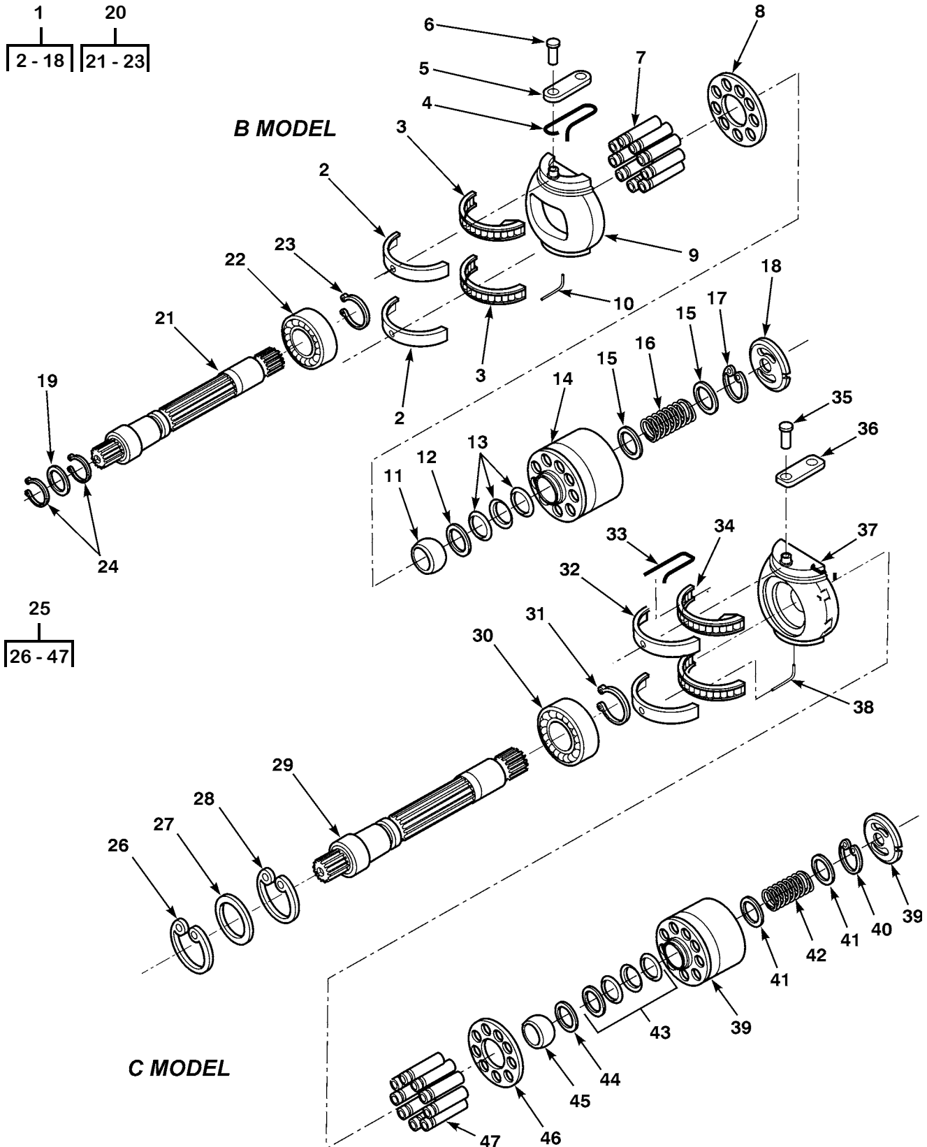
Figure 72. Rotary Pump
