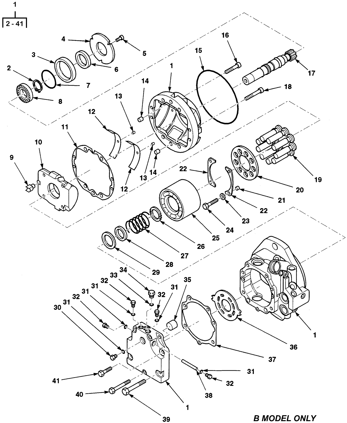
Figure 66. Front Propel Motor Assembly (Sheet 1 of 2)
