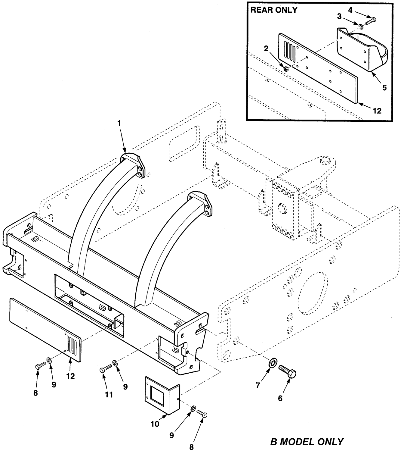
Figure 96. Bumper Assemblies (Sheet 1 of 2)
