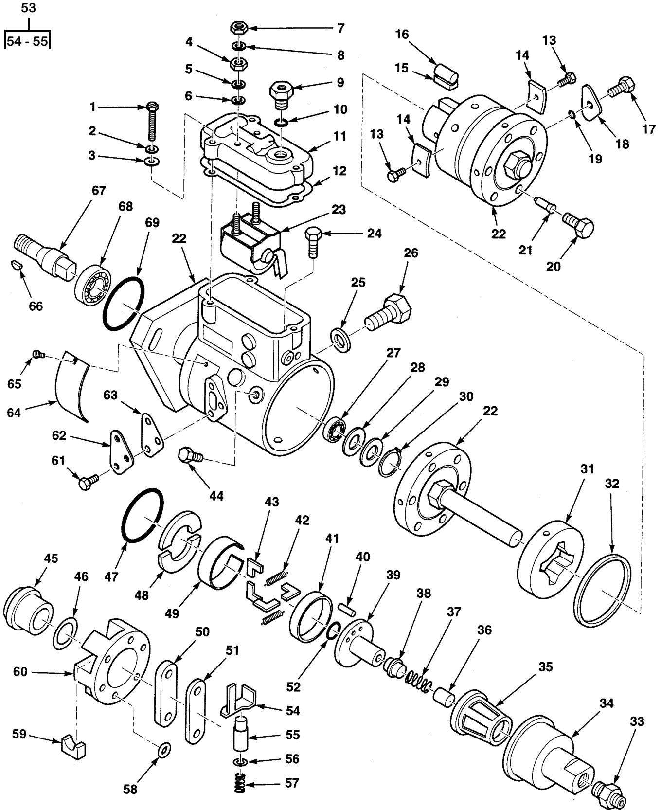
Figure 21. Fuel Injector Pump (Internal), B Model Only
