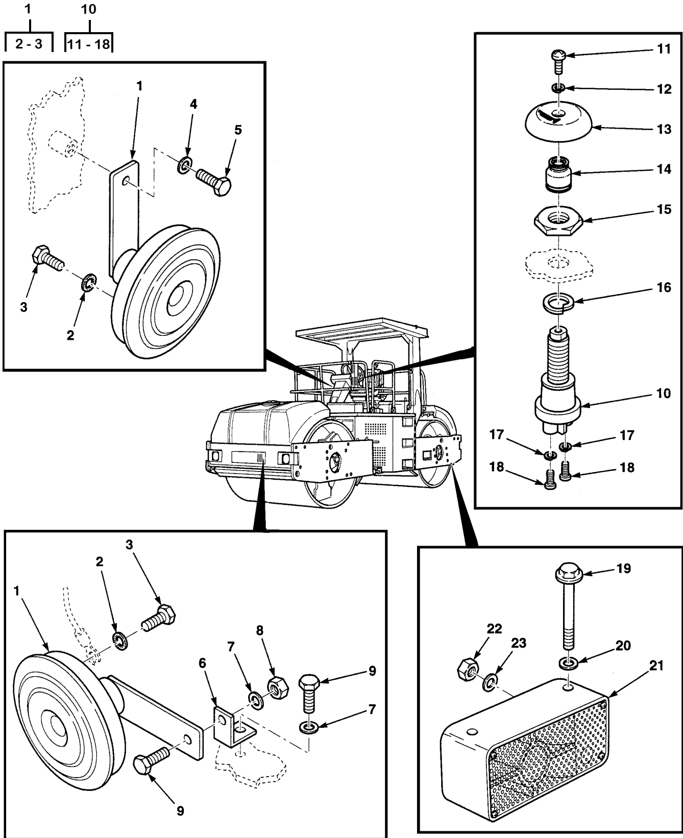
Figure 53. Horn and Backup Alarm
