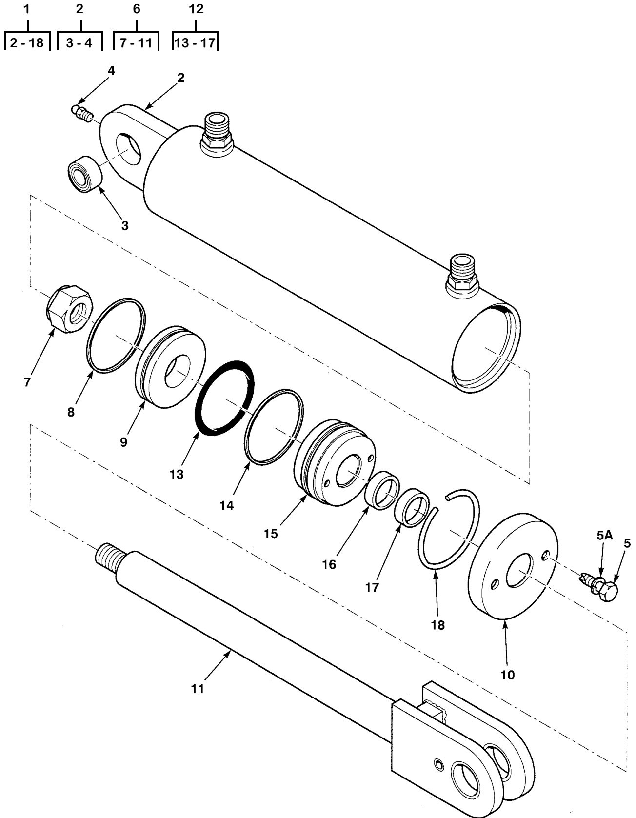
Figure 93. Hydraulic Steering Cylinder
