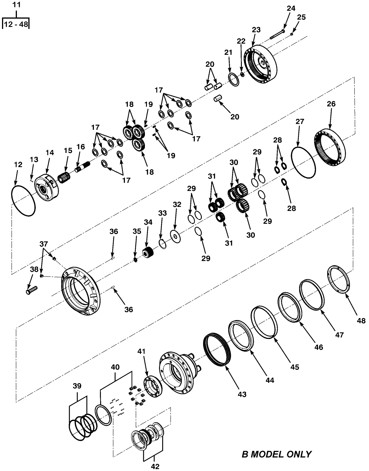
Figure 80. Front Propel Gearbox Assembly (Sheet 2 of 3)
