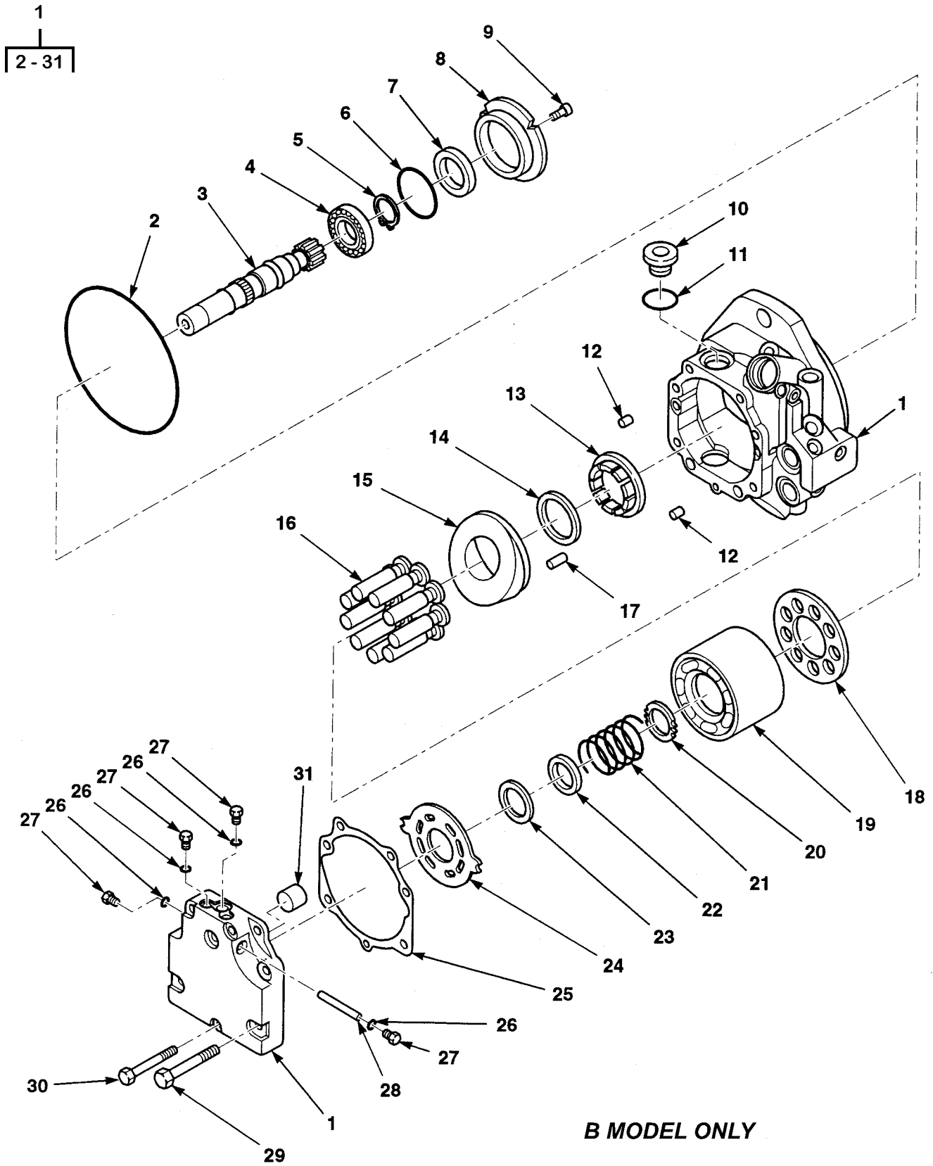
Figure 69. Rear Propeller Piston Motor (Sheet 1 of 2)
