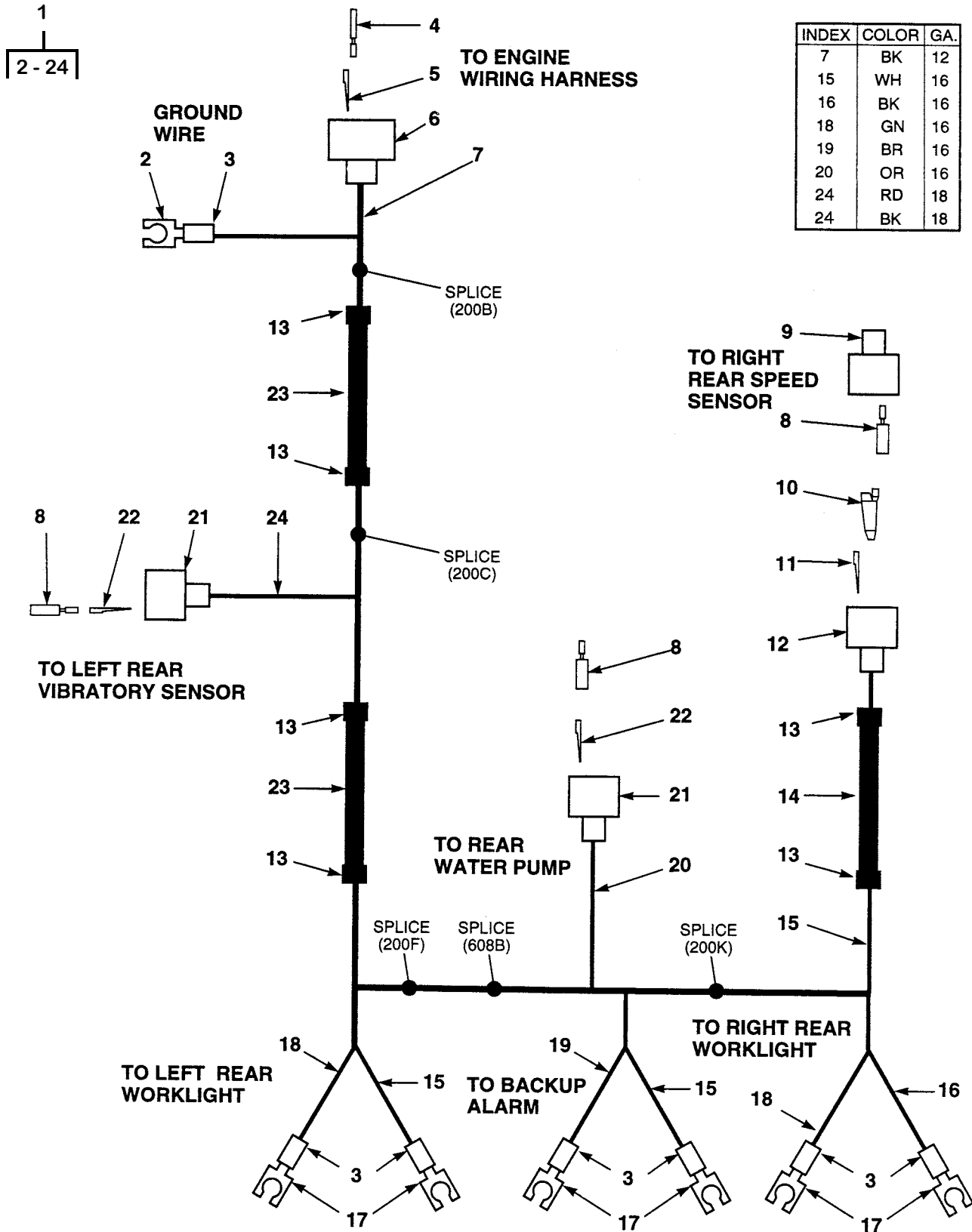
Figure 60. Rear Wiring Harness
