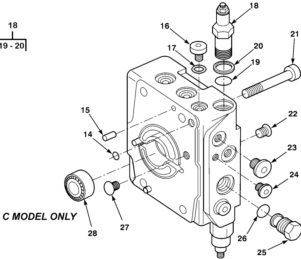
Figure 117. Vibratory Port Block Assembly
