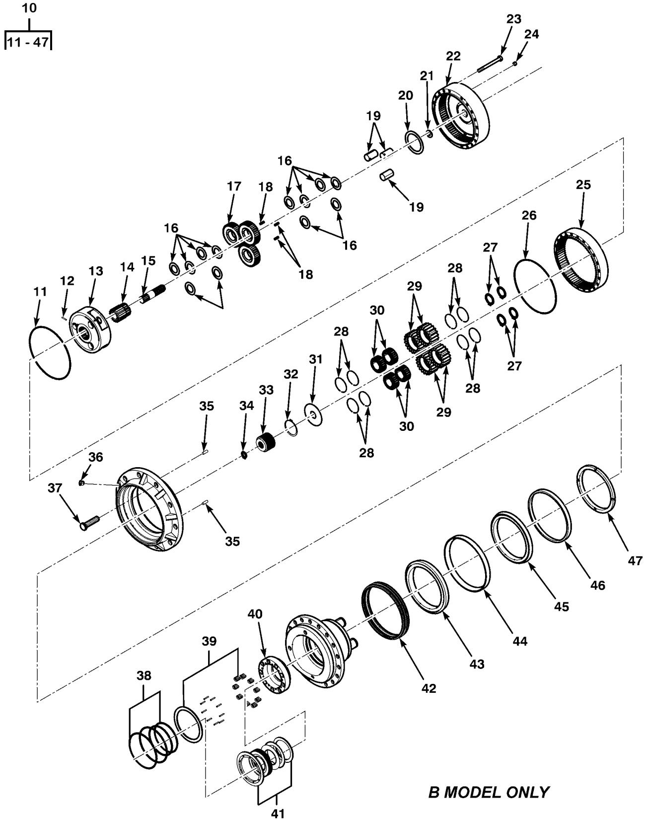
Figure 79. Rear Propeller Gearbox Assembly (Sheet 2 of 3)
