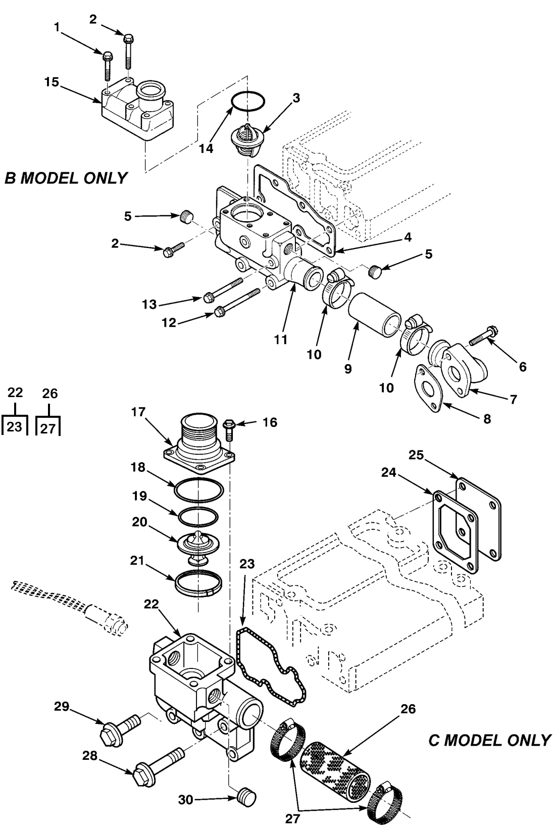
Figure 39. Thermostat, Housing, Hoses and Fittings
