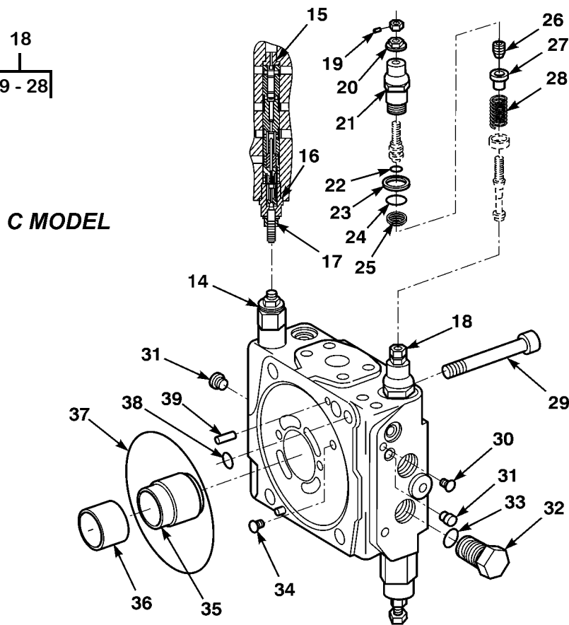
Figure 75. Port Block Assembly
