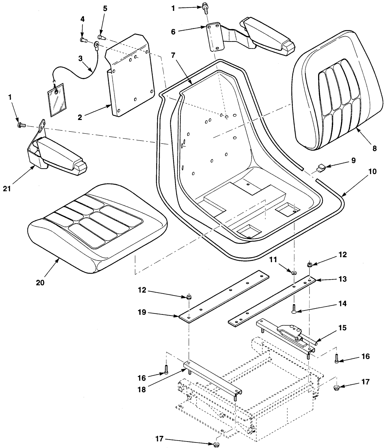
Figure 106. Seat Assembly Components
