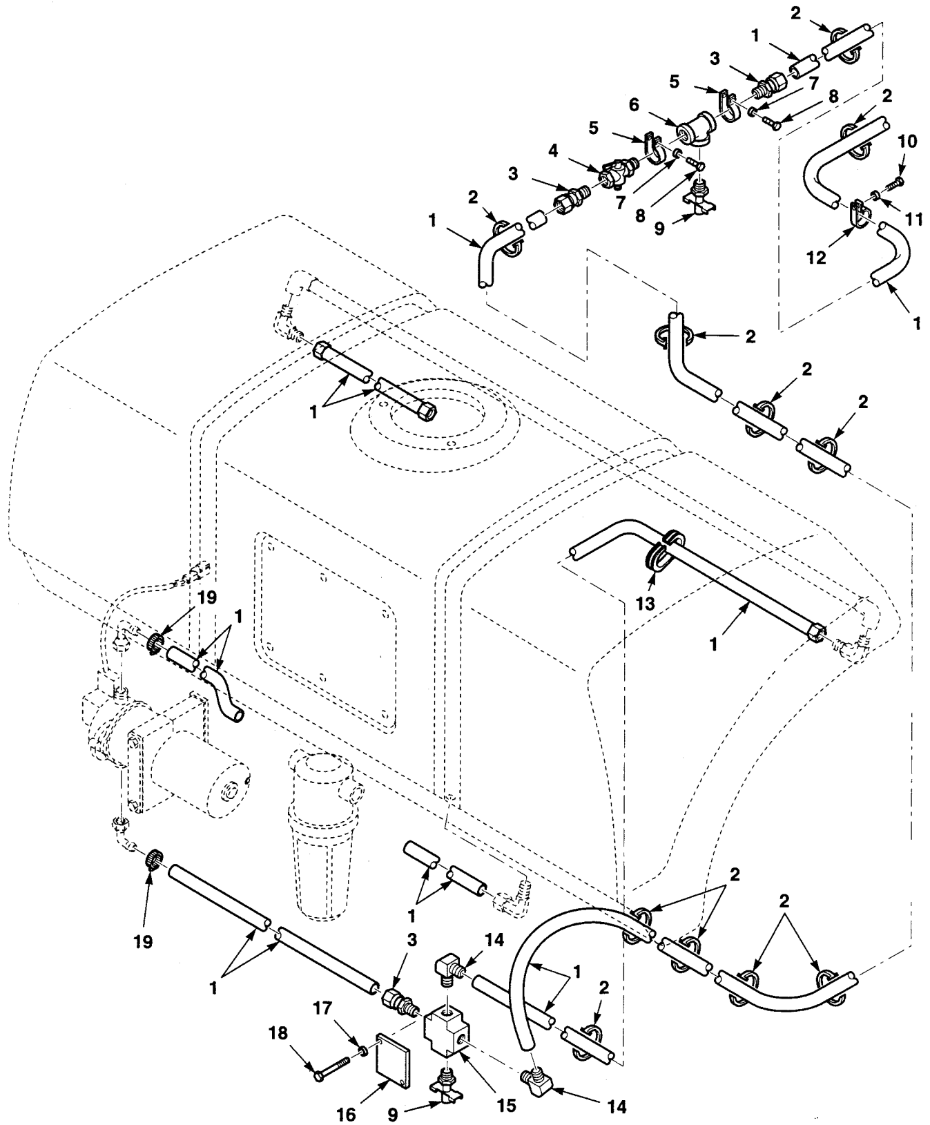
Figure 137. Water Spray Tubes and Fittings
