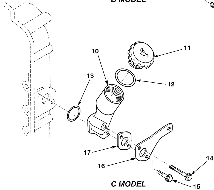
Figure 13. Engine Oil Filler
