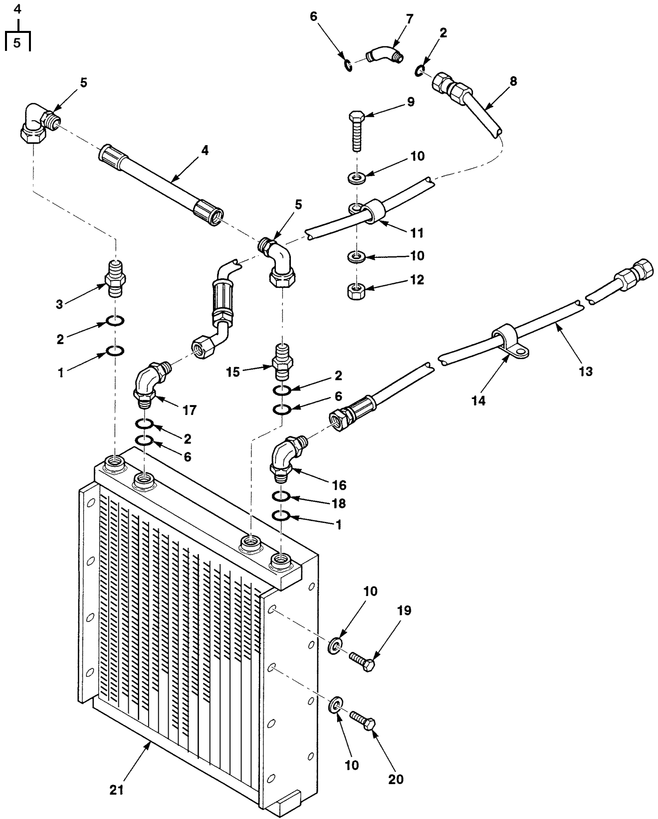
Figure 127. Hydraulic Oil Cooler, Hoses and Fittings
