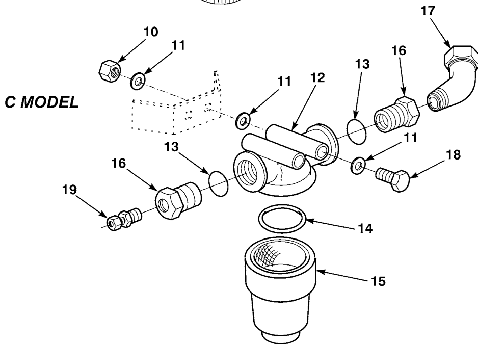
Figure 138. Water Screen Assemblies
