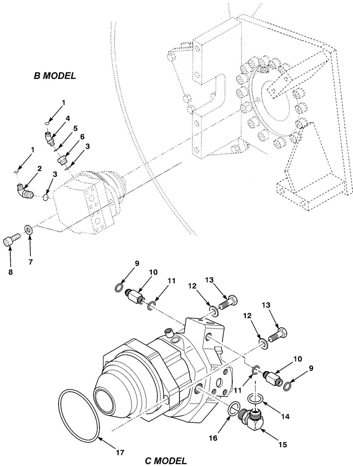
Figure 68. Rear Propel Motor Mounting
