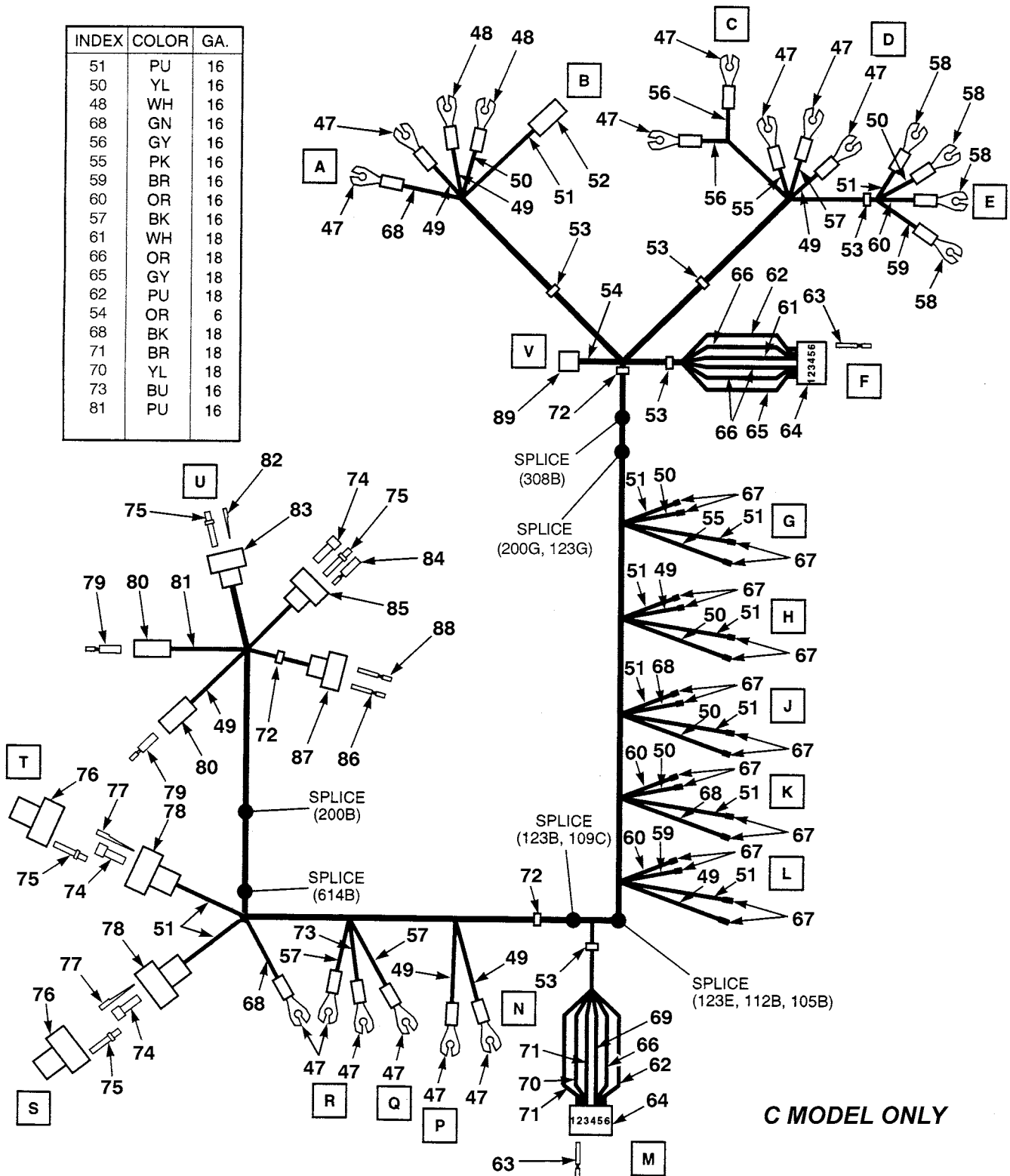
Figure 62. Instrument Harness Assembly (Sheet 3 of 3)
