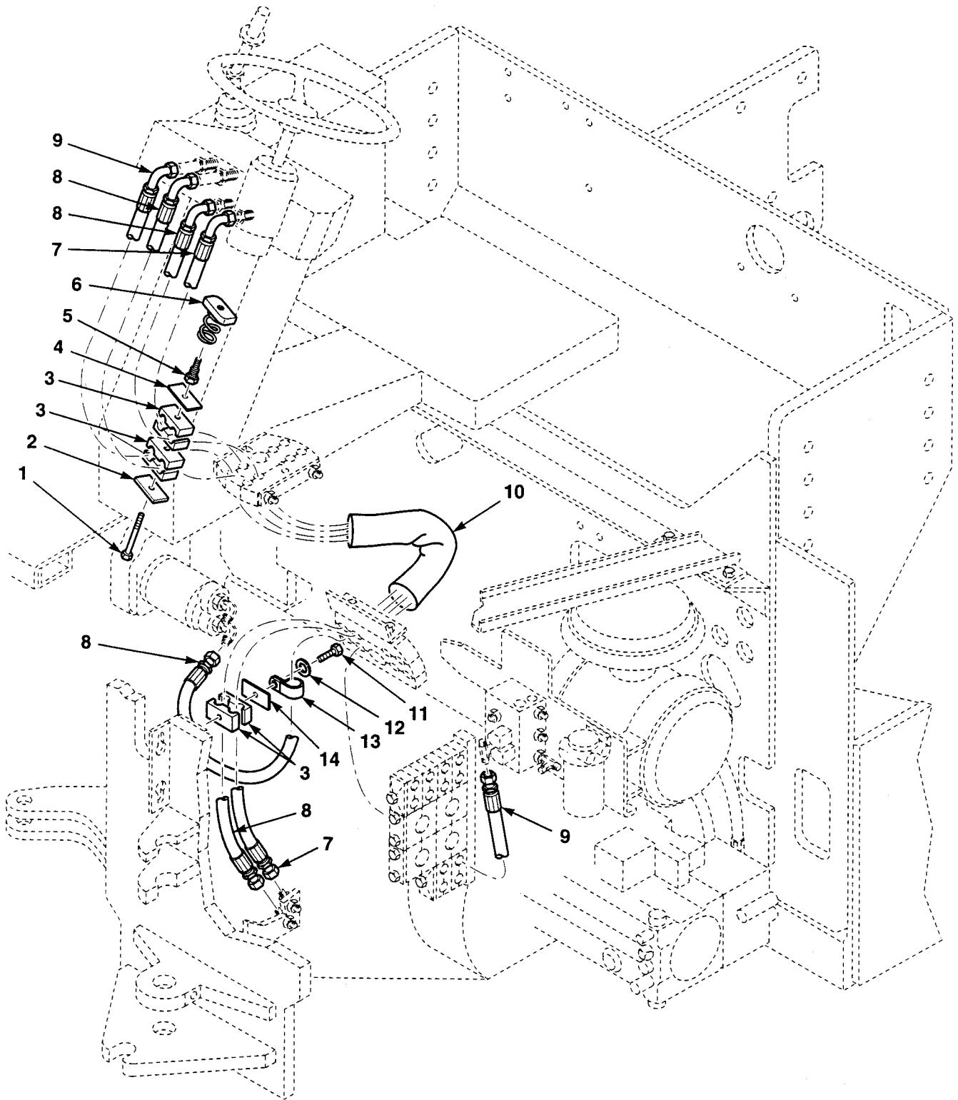
Figure 90. Steering Lines and Fittings
