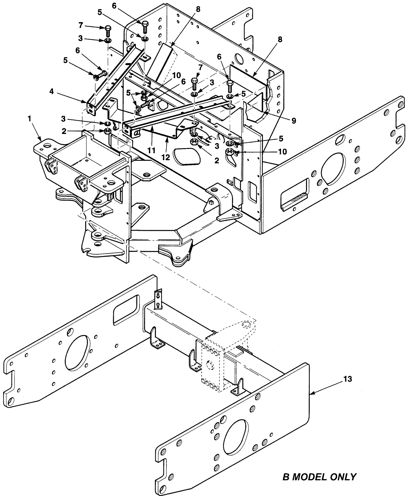
Figure 95. Roller Frame (Sheet 1 of 2)
