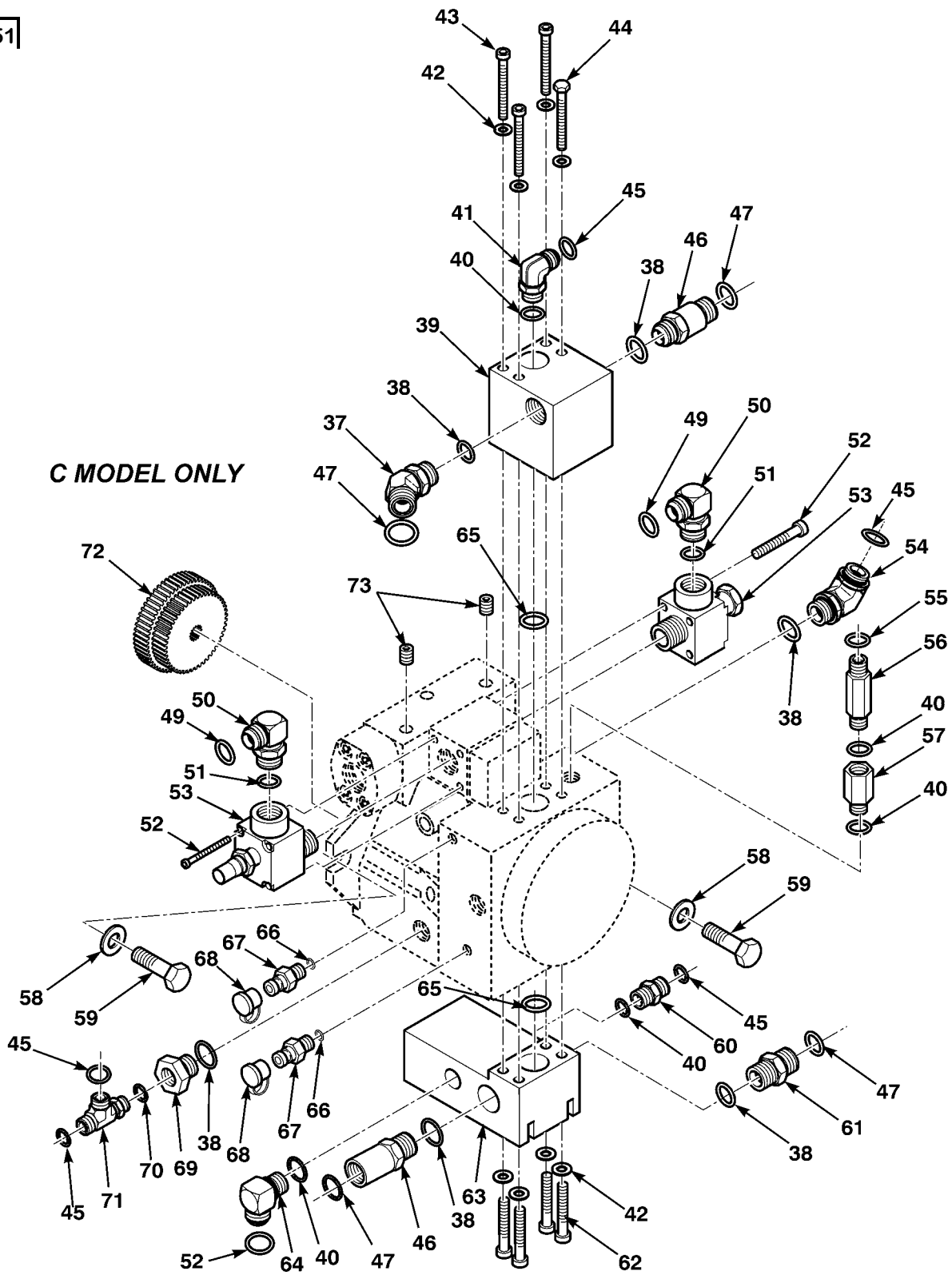
Figure 70. Hydraulic Propel Pump Mounting (Sheet 2 of 2)
