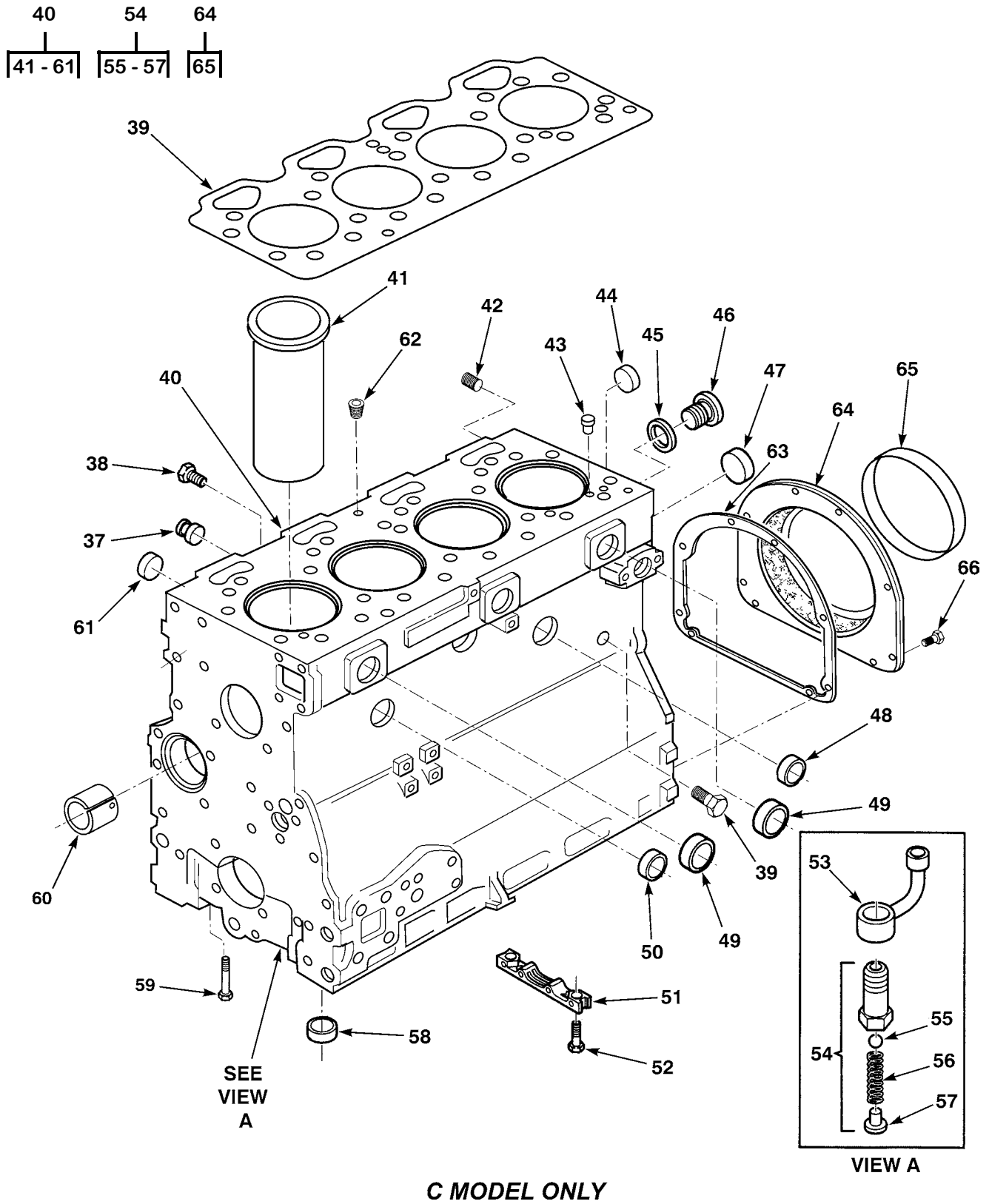
Figure 2. Cylinder Block Assembly (Sheet 2 of 2)
