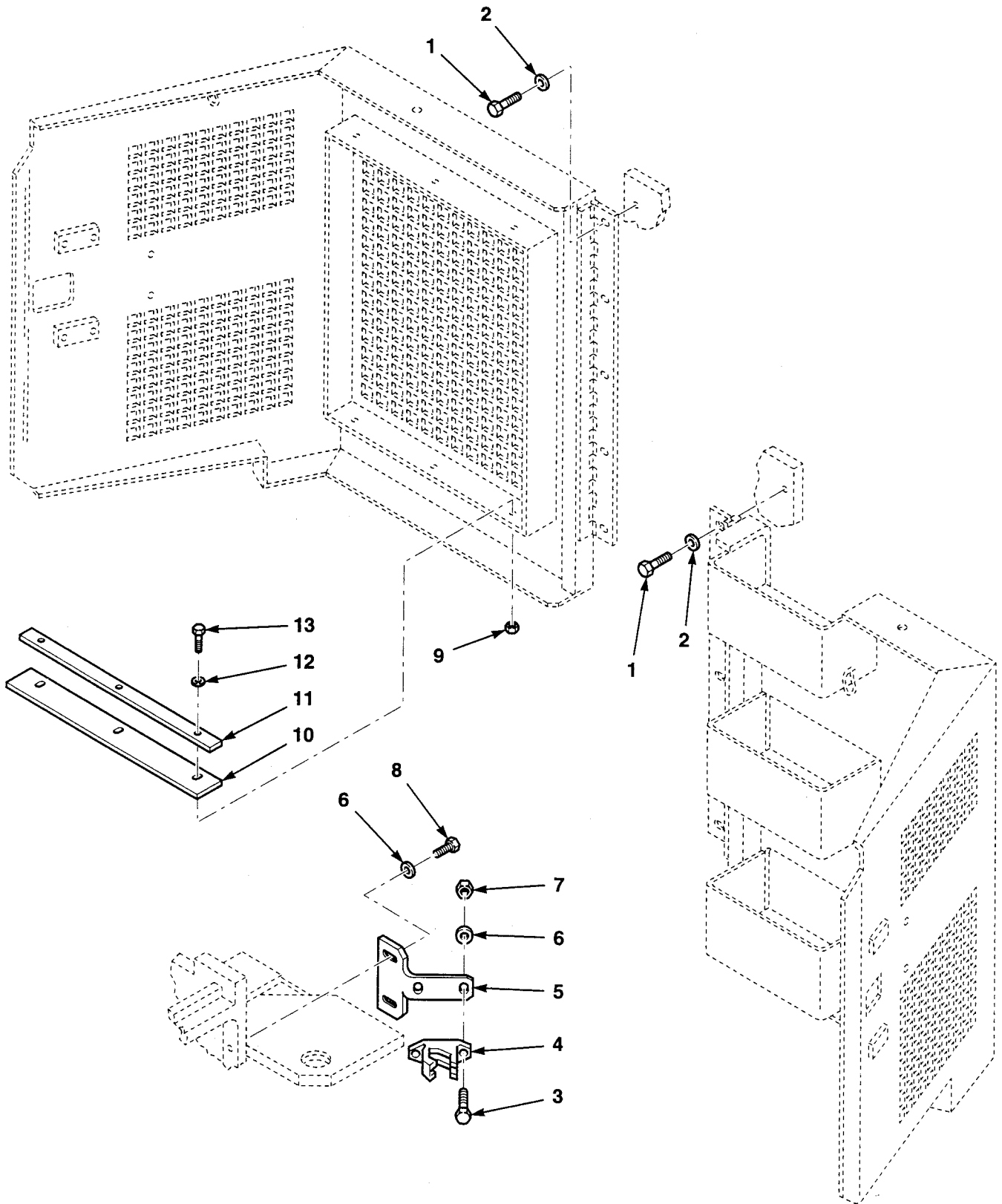
Figure 99. Door Assemblies Mounting
