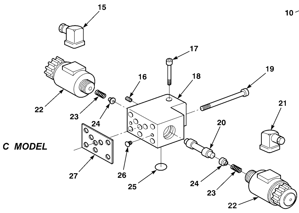
Figure 113. Vibratory Control and Solenoids Assembly
