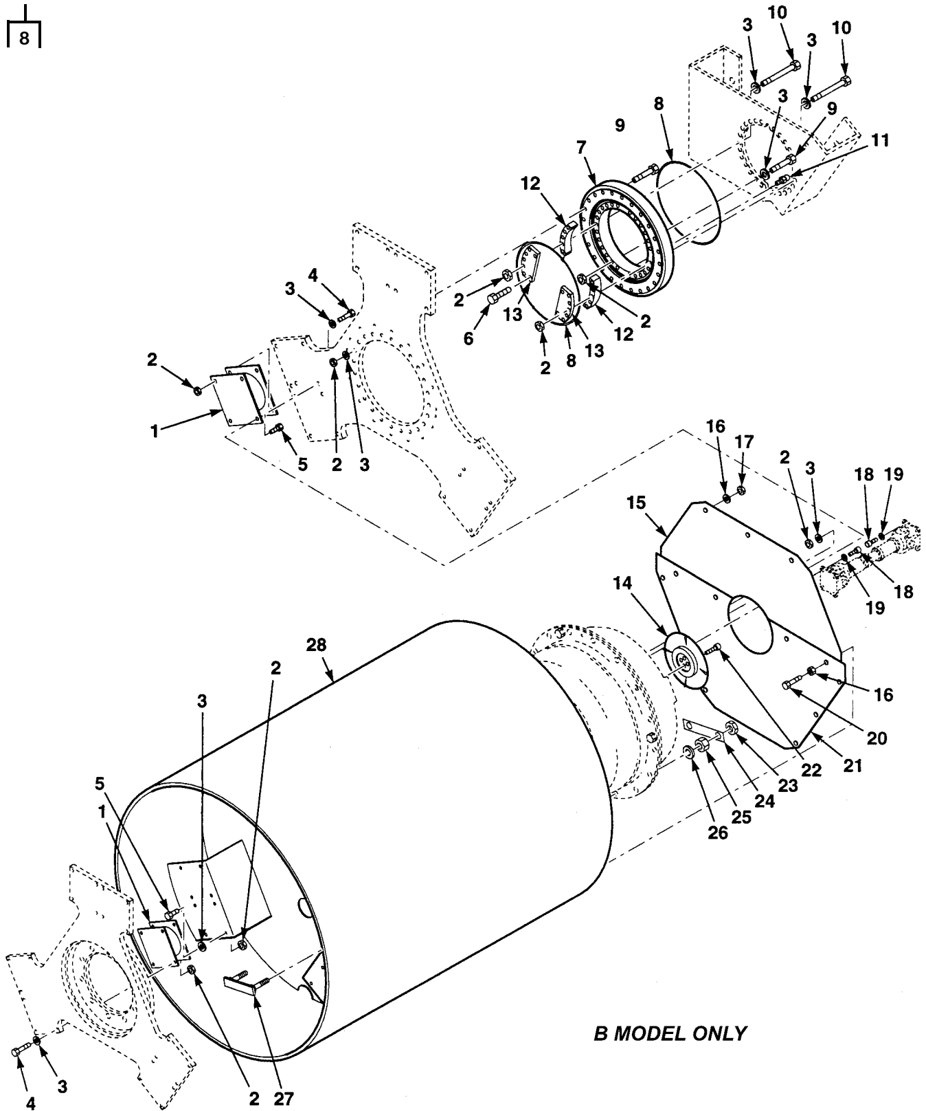
Figure 133. Front and Rear Drum Assemblies and Mounts (Sheet 1 of 2)
