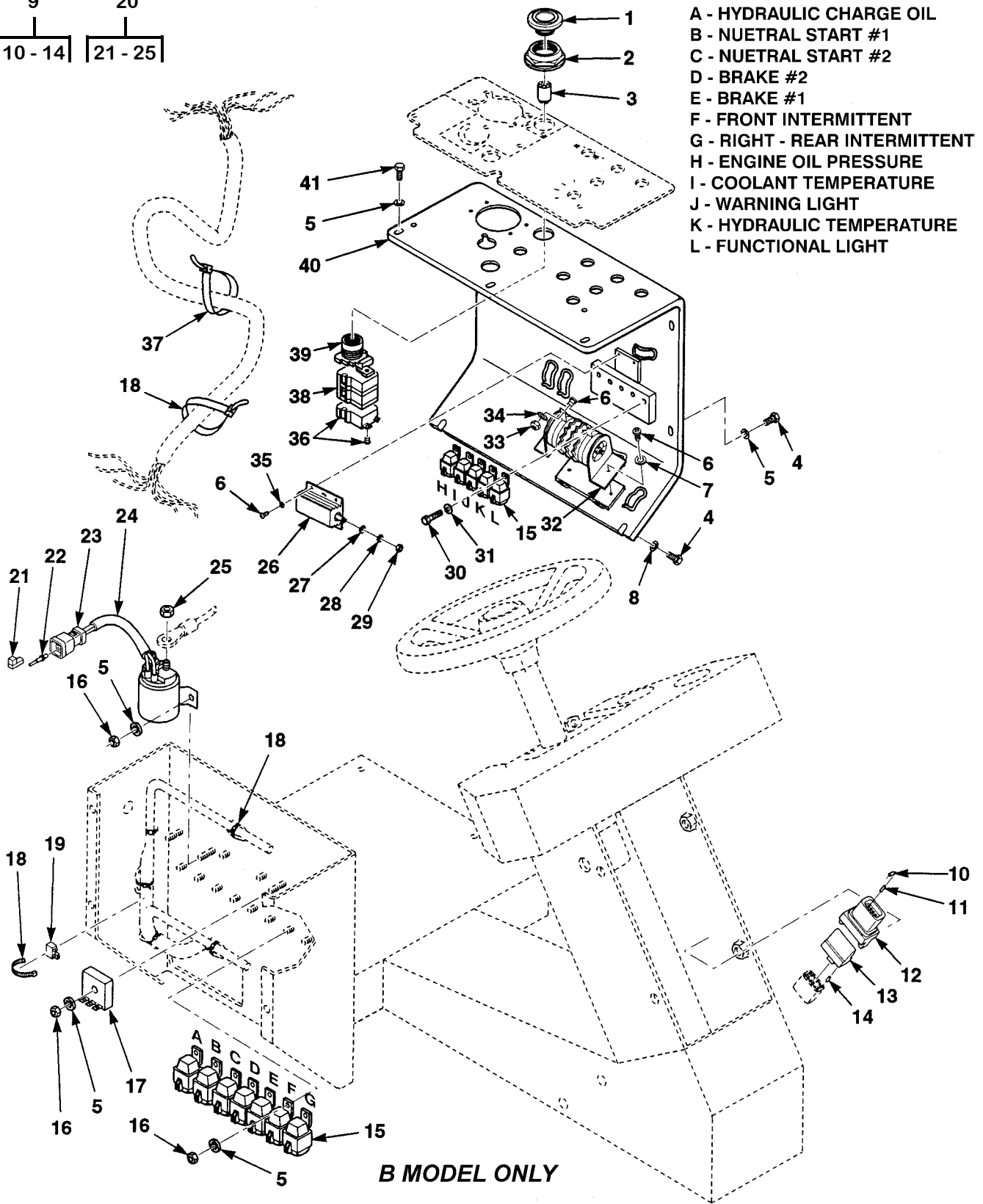
Figure 50. Switches and Relays (Sheet 1 of 2)
