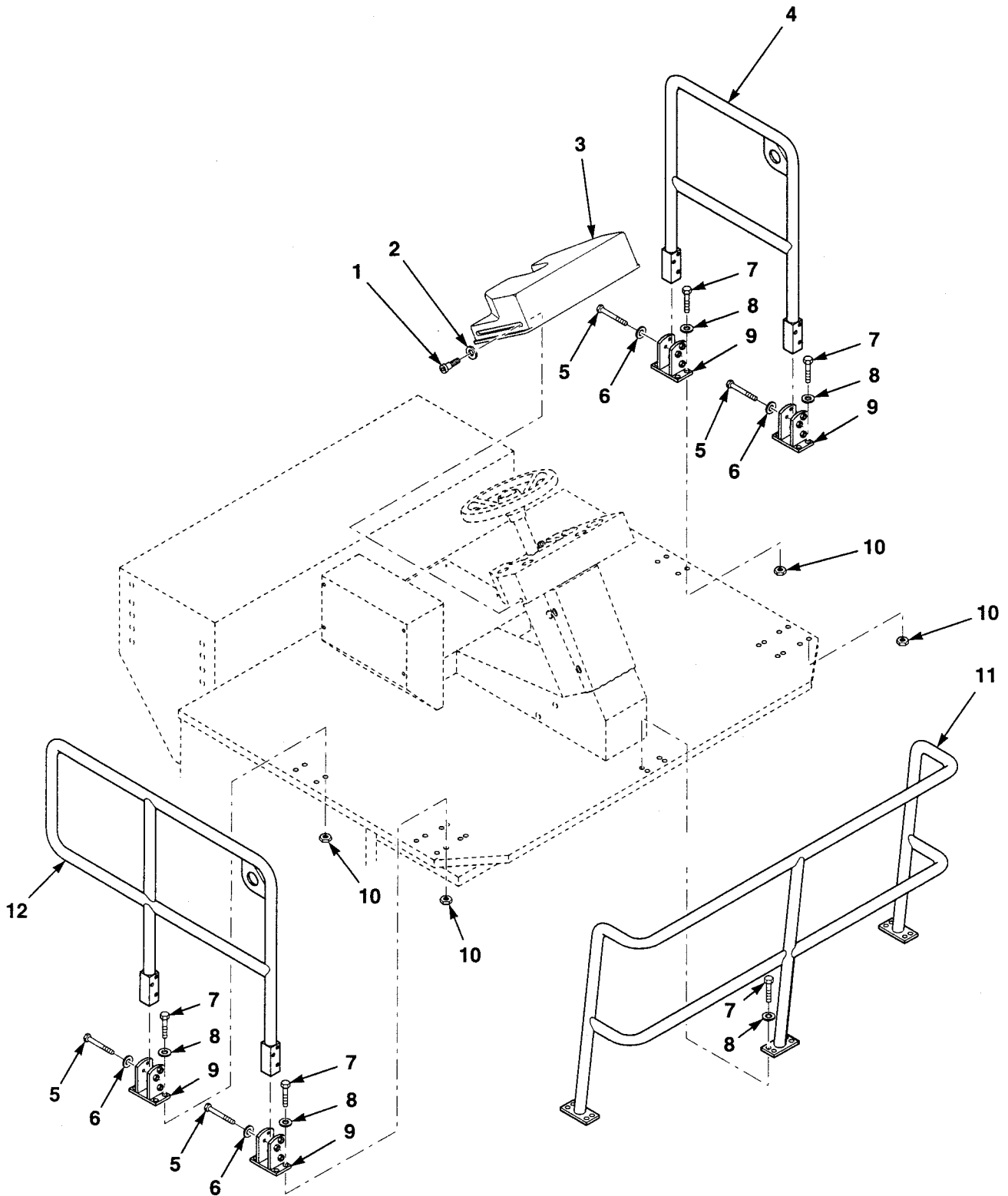
Figure 103. Vandal Guard and Handrails
