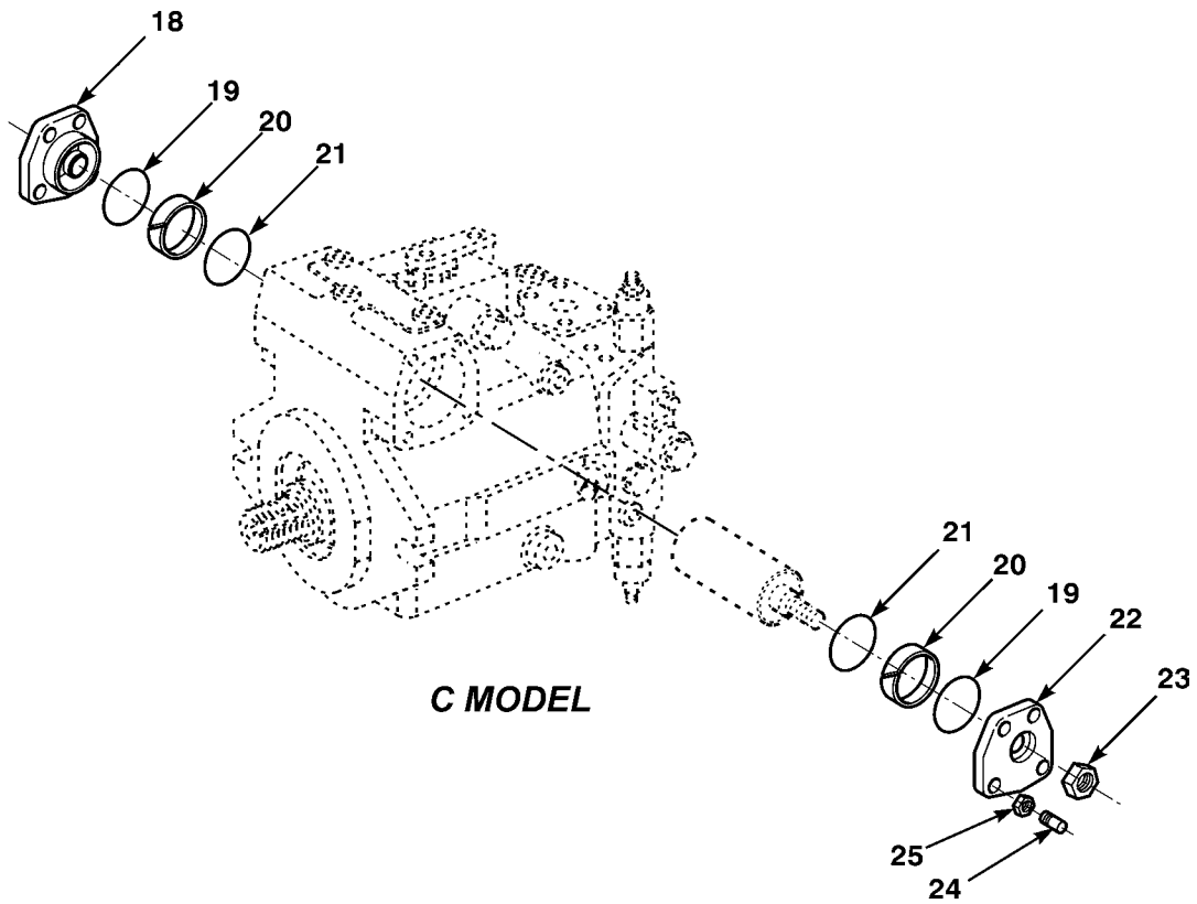
Figure 73. Shaft and Housing Assembly
