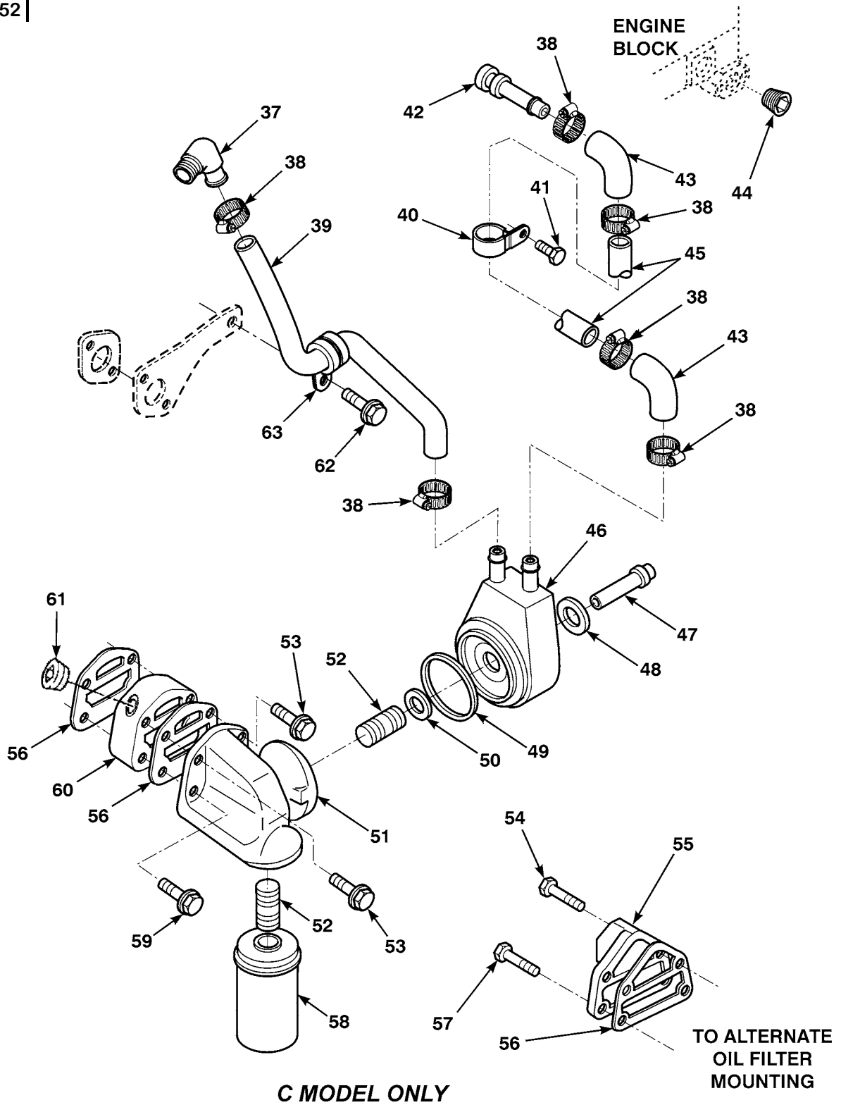
Figure 15. Engine Oil Filter and Cooler Assembly (Sheet 2 of 2)
