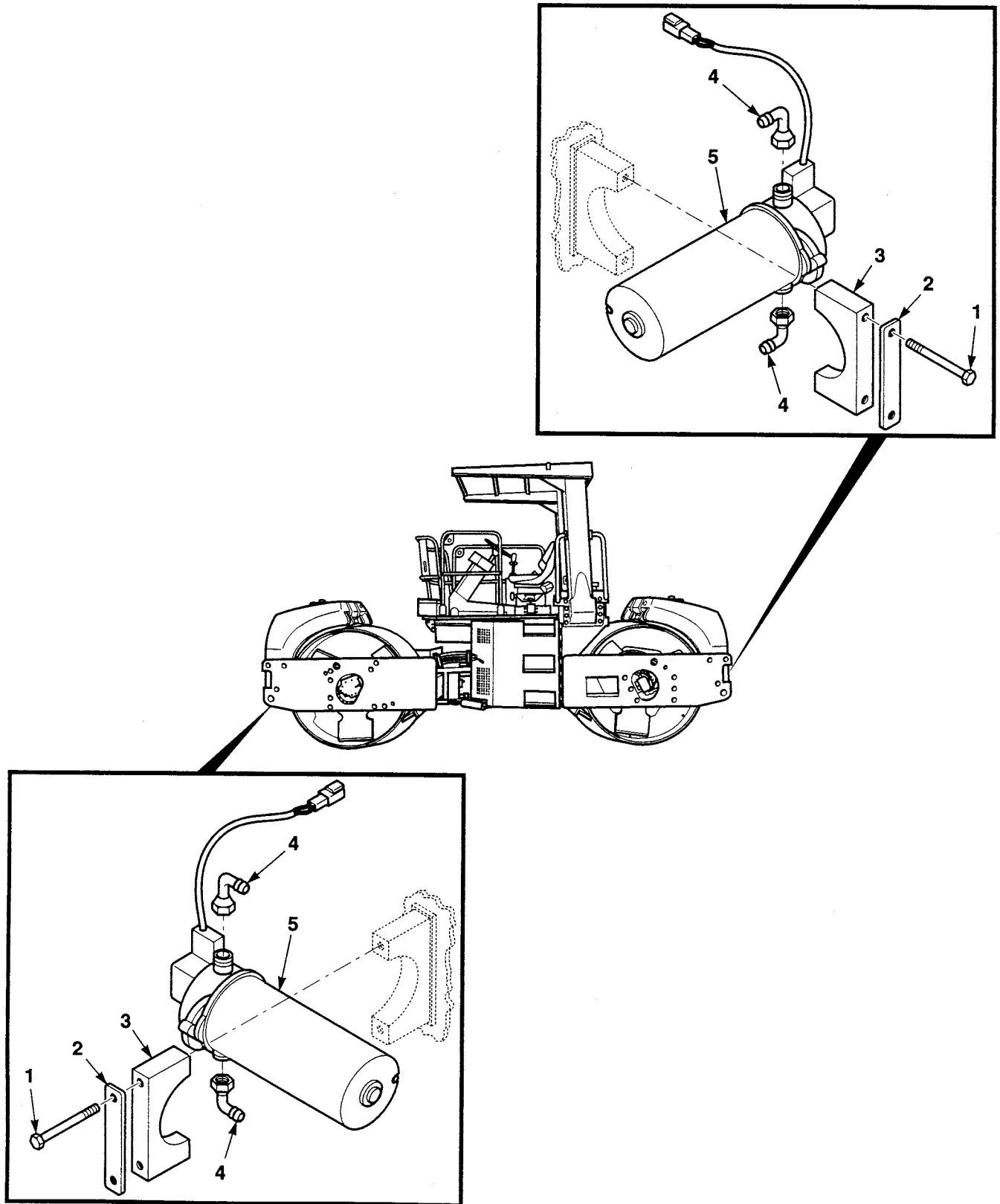
Figure 135. Front and Rear Water Spray Pumps
