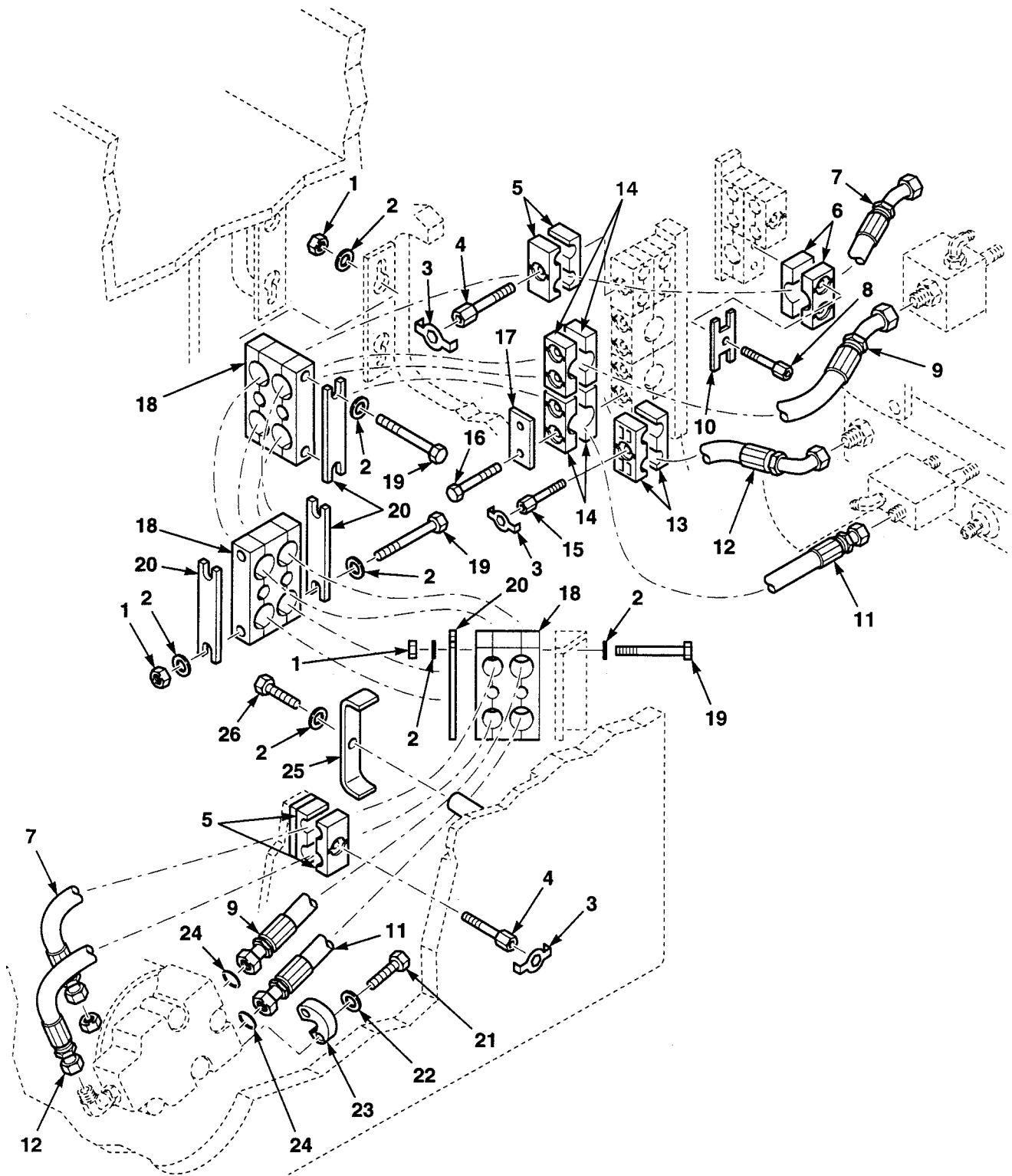
Figure 124. Front Hydraulic Lines and Fittings
