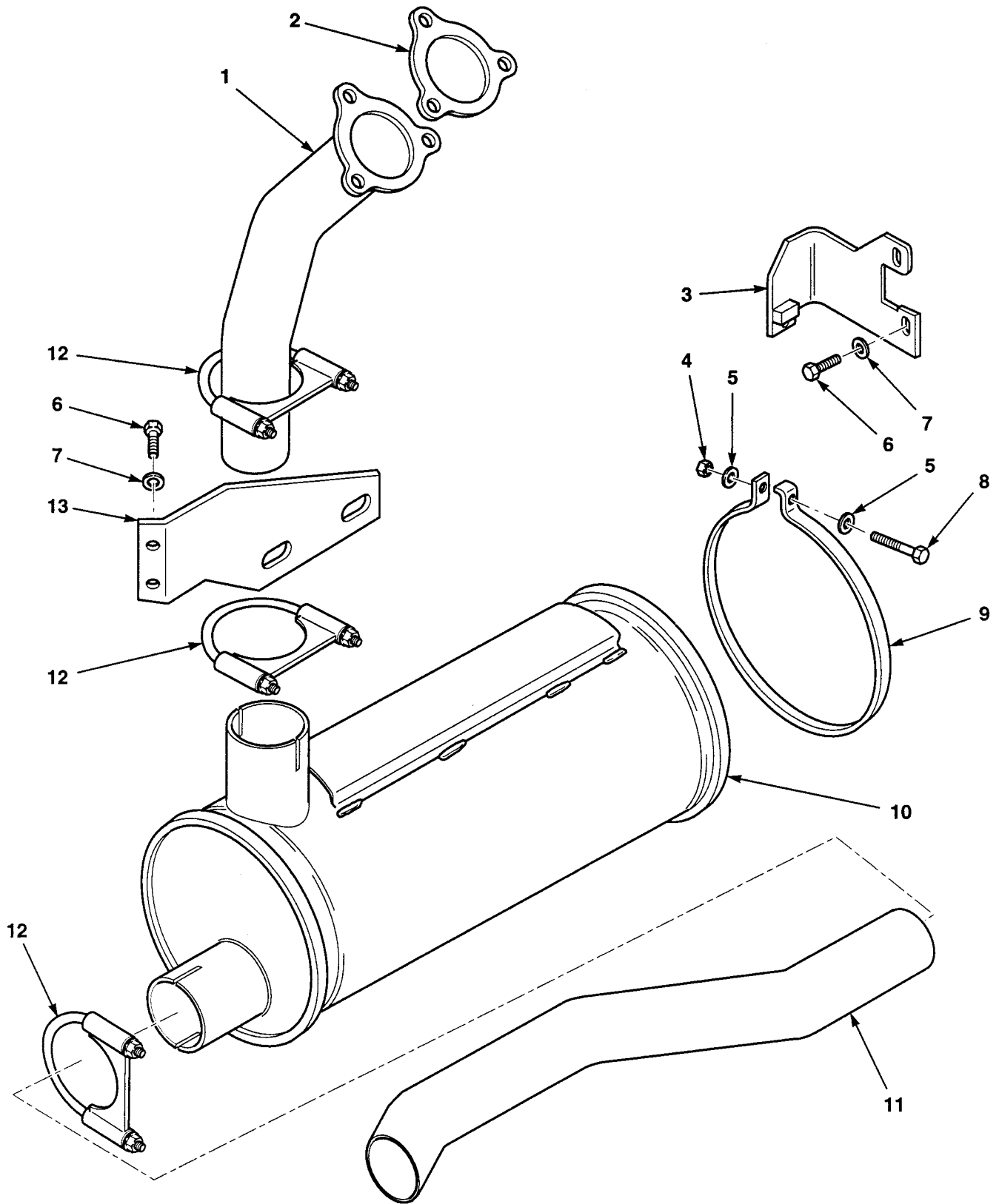
Figure 36. Muffler and Exhaust System
