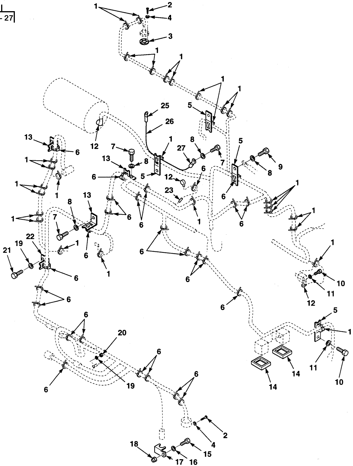
Figure 56. Engine Wiring Harness Mounting Hardware
