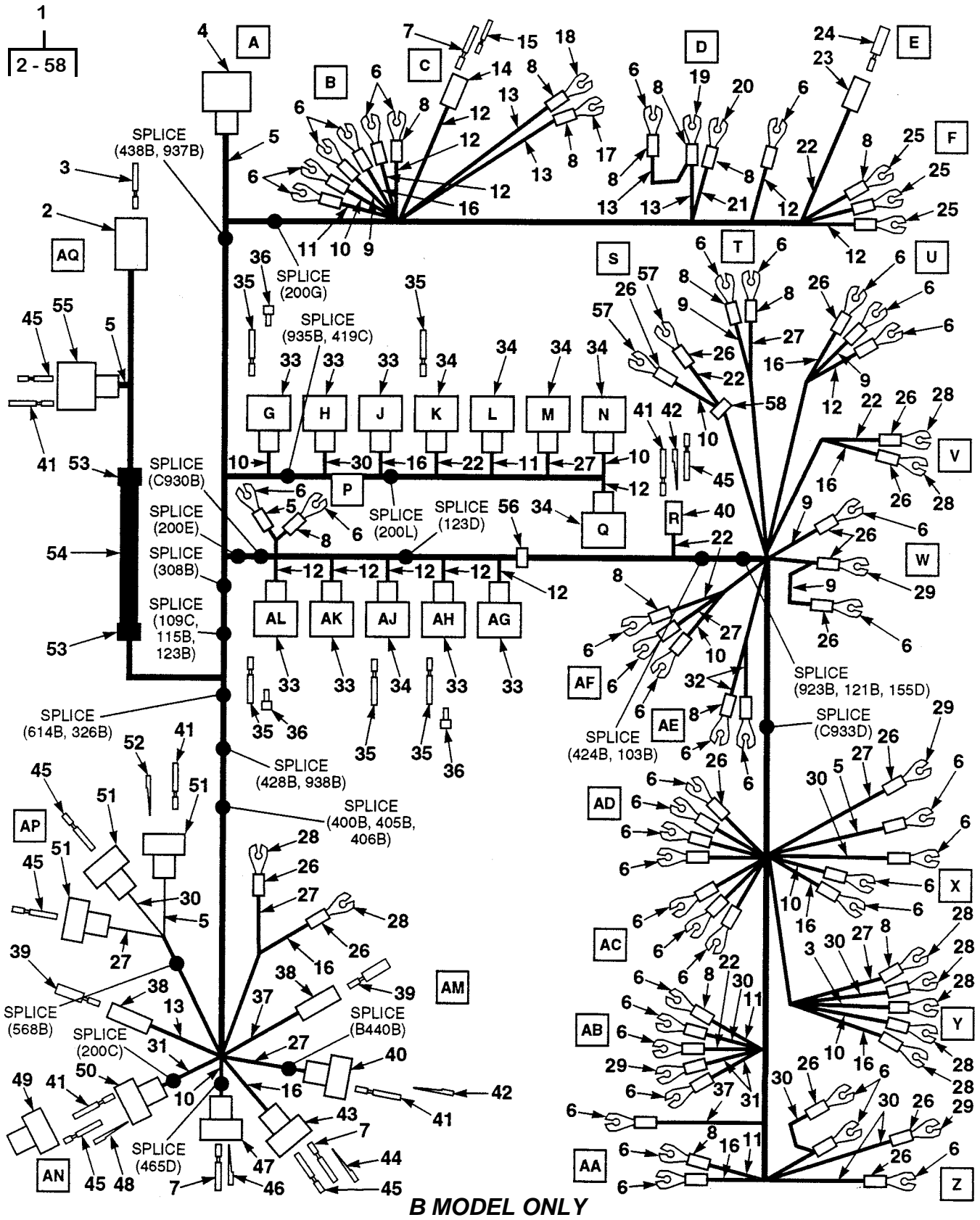
Figure 63. Main Wiring Harness (Sheet 1 of 3)
