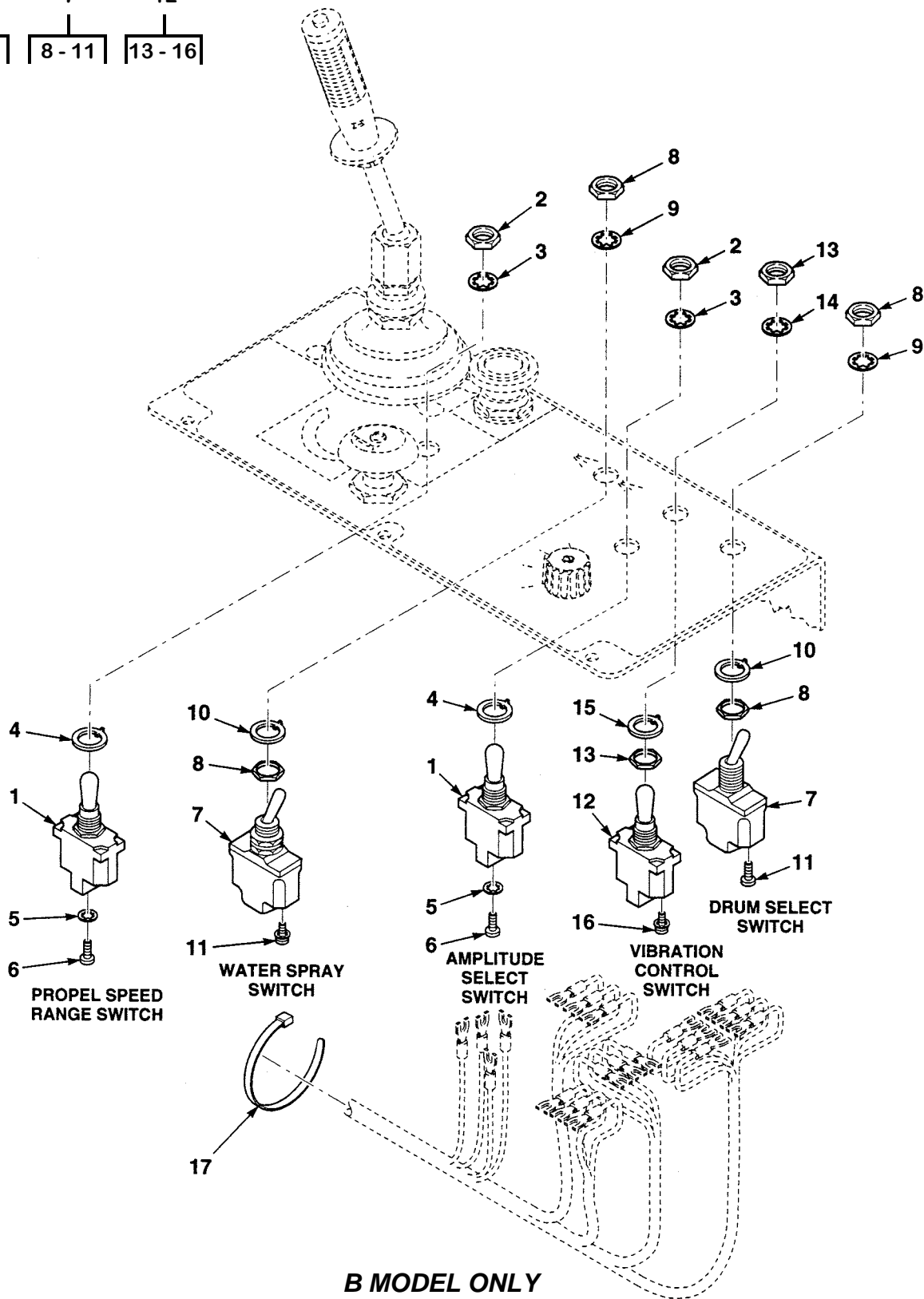
Figure 49. Switches (Sheet 1 of 2)
