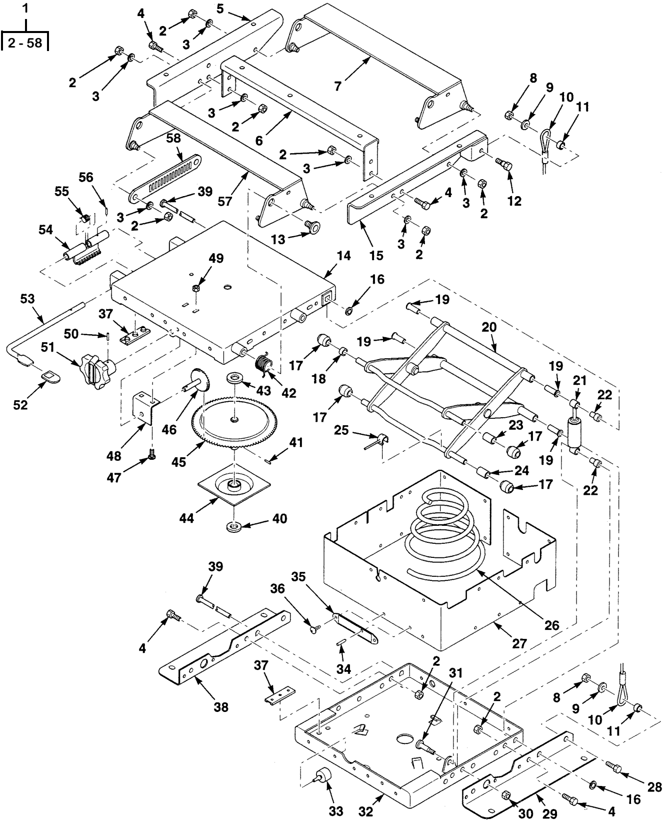
Figure 107. Seat Suspension Assembly
