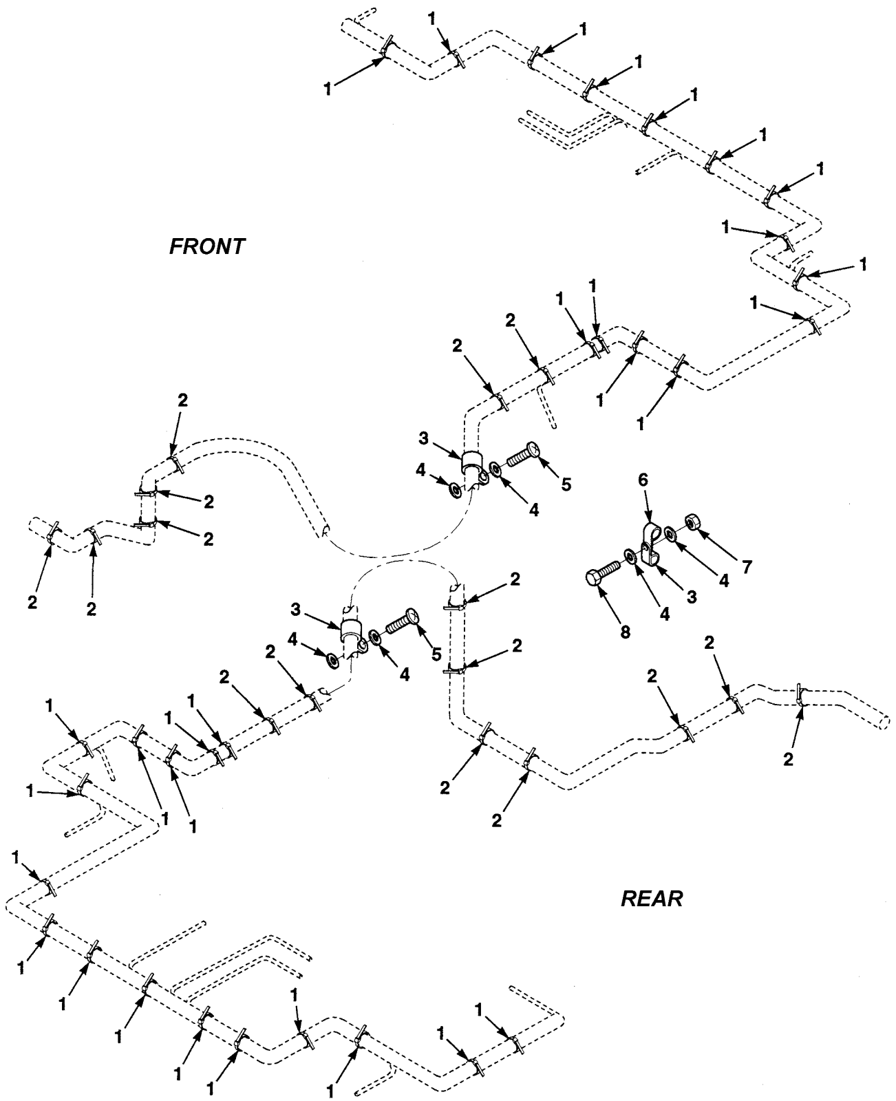
Figure 58. Front and Rear Wiring Harness Mounting Hardware
