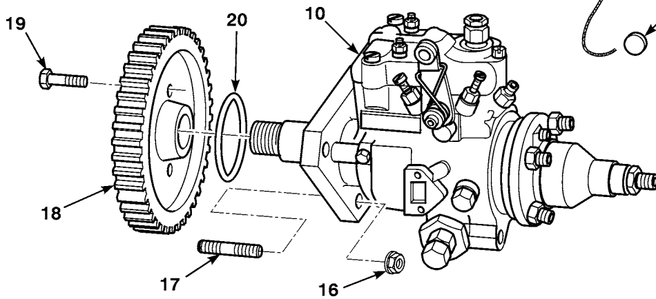
Figure 20. Fuel Injector Pump and Gear
