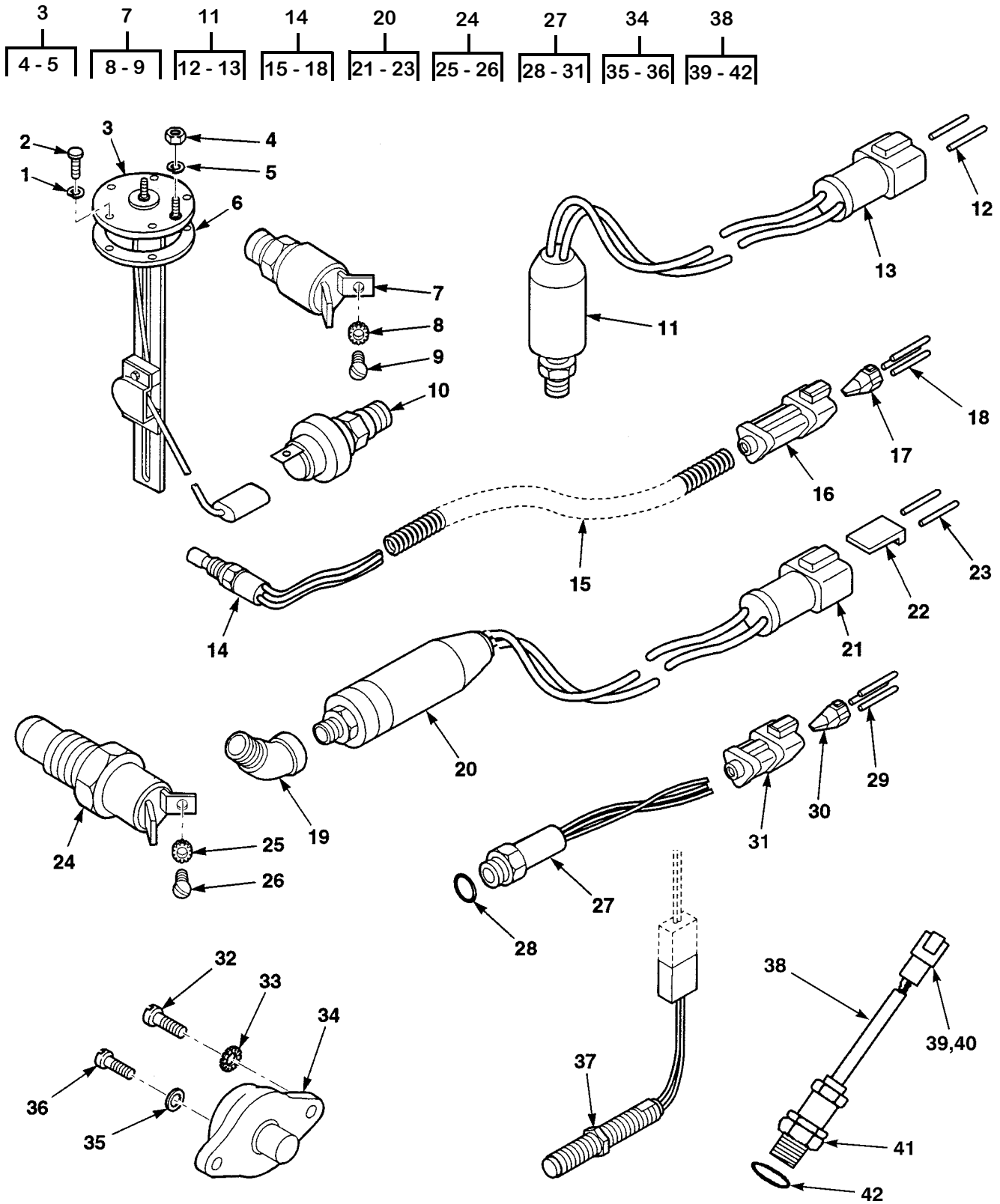
Figure 52. Switches, Sending Units and Circuit Breakers
