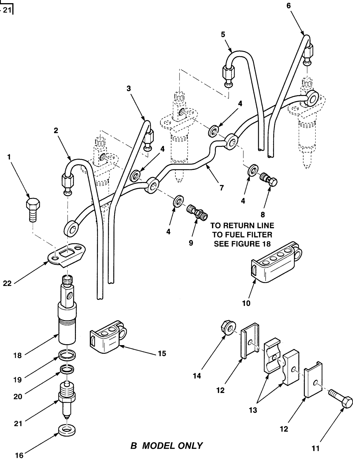
Figure 17. Fuel Injector Assembly, Lines and Fittings (Sheet 1 of 2)
