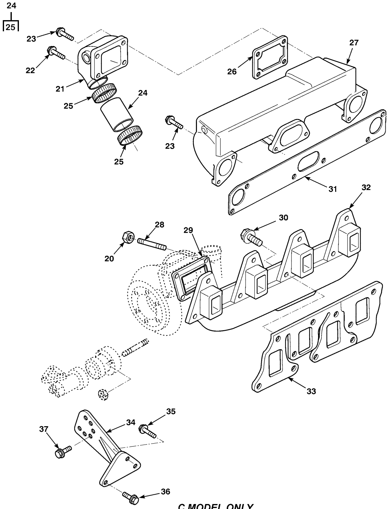
Figure 16. Intake and Exhaust Manifolds and Turbocharger Lines (Sheet 2 of 2)
