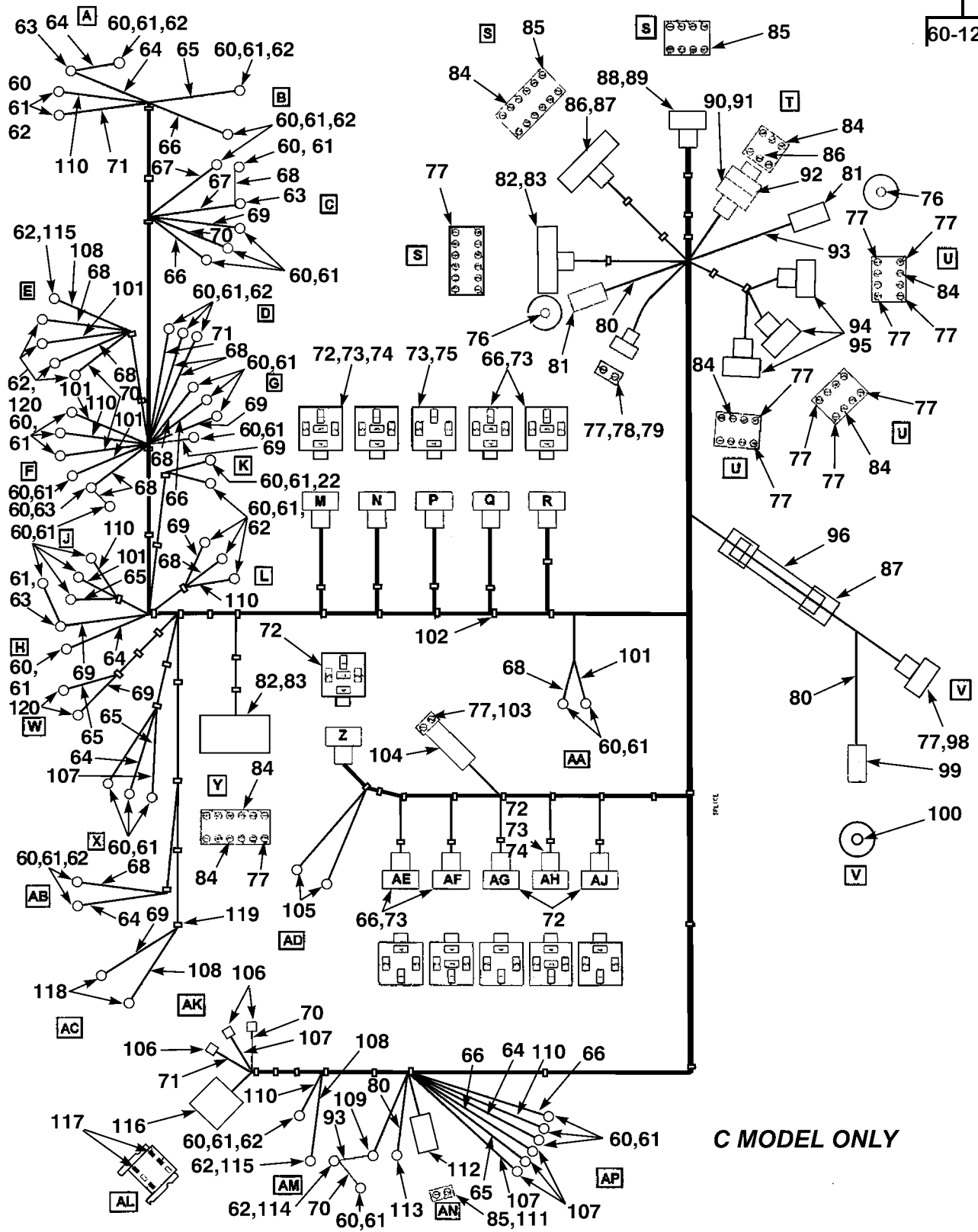
Figure 63. Main Wiring Harness (Sheet 3 of 3)
