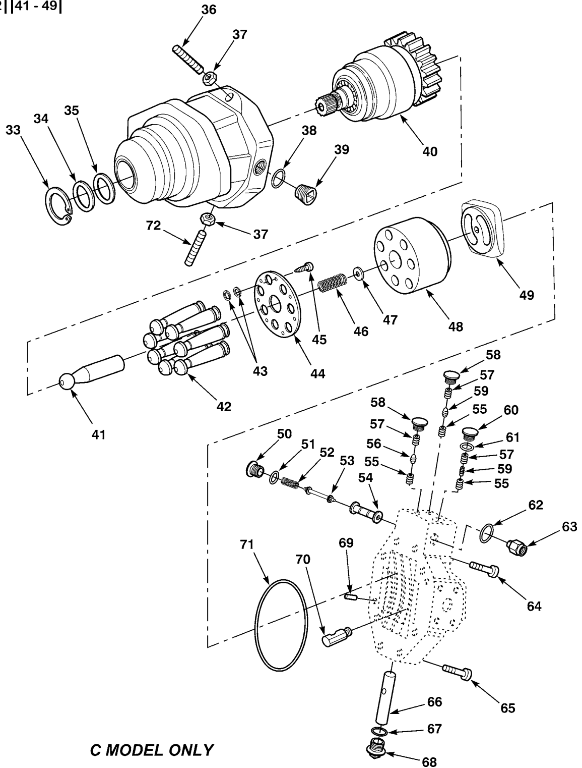
Figure 69. Rear Propeller Piston Motor (Sheet 2 of 2)
