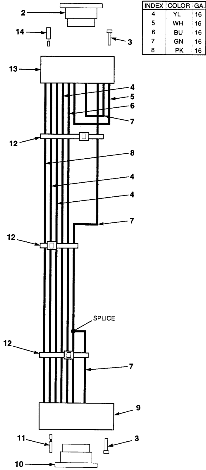
Figure 61. Operator Control Interface Harness
