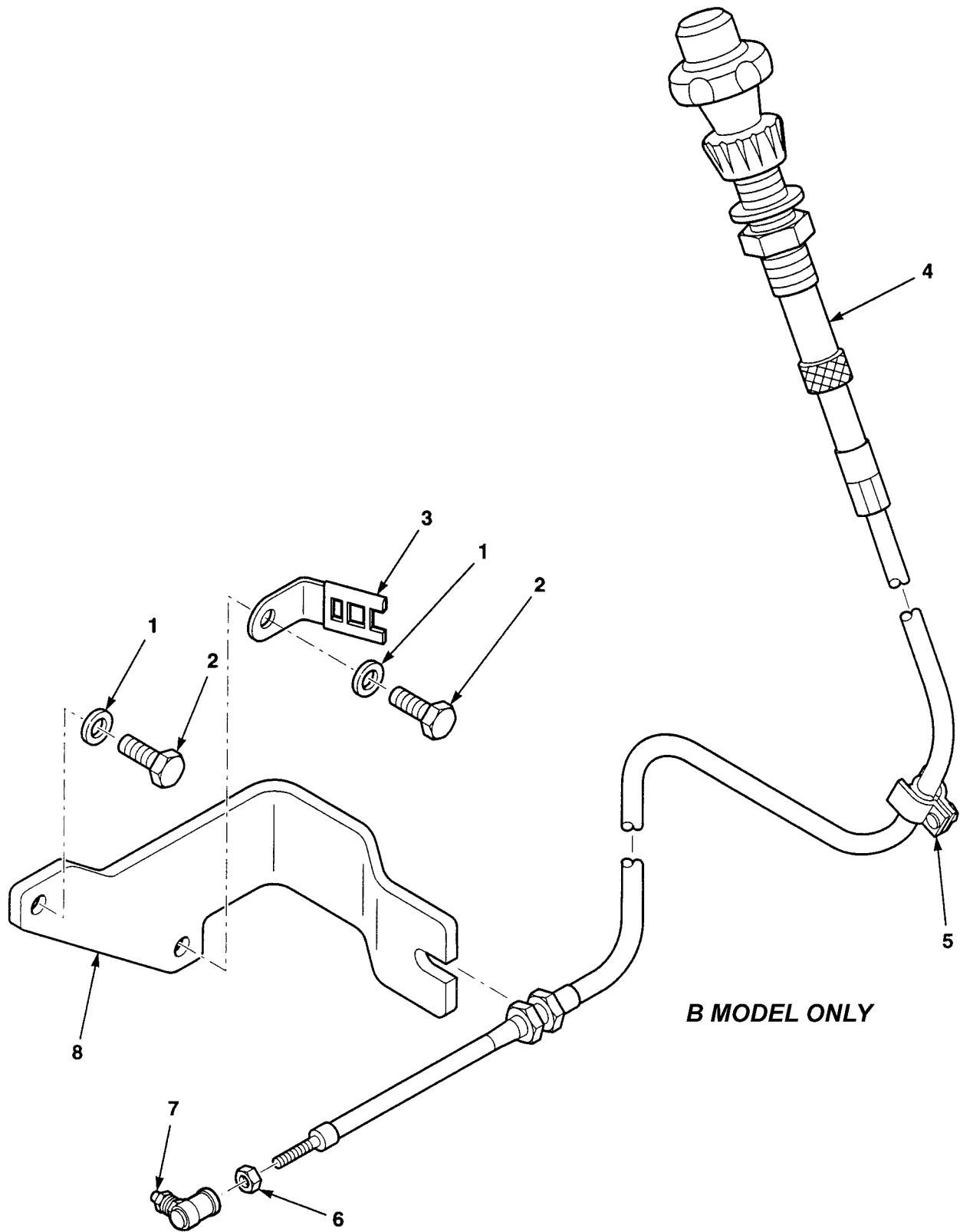
Figure 35. Throttle Control (Sheet 1 of 2)
