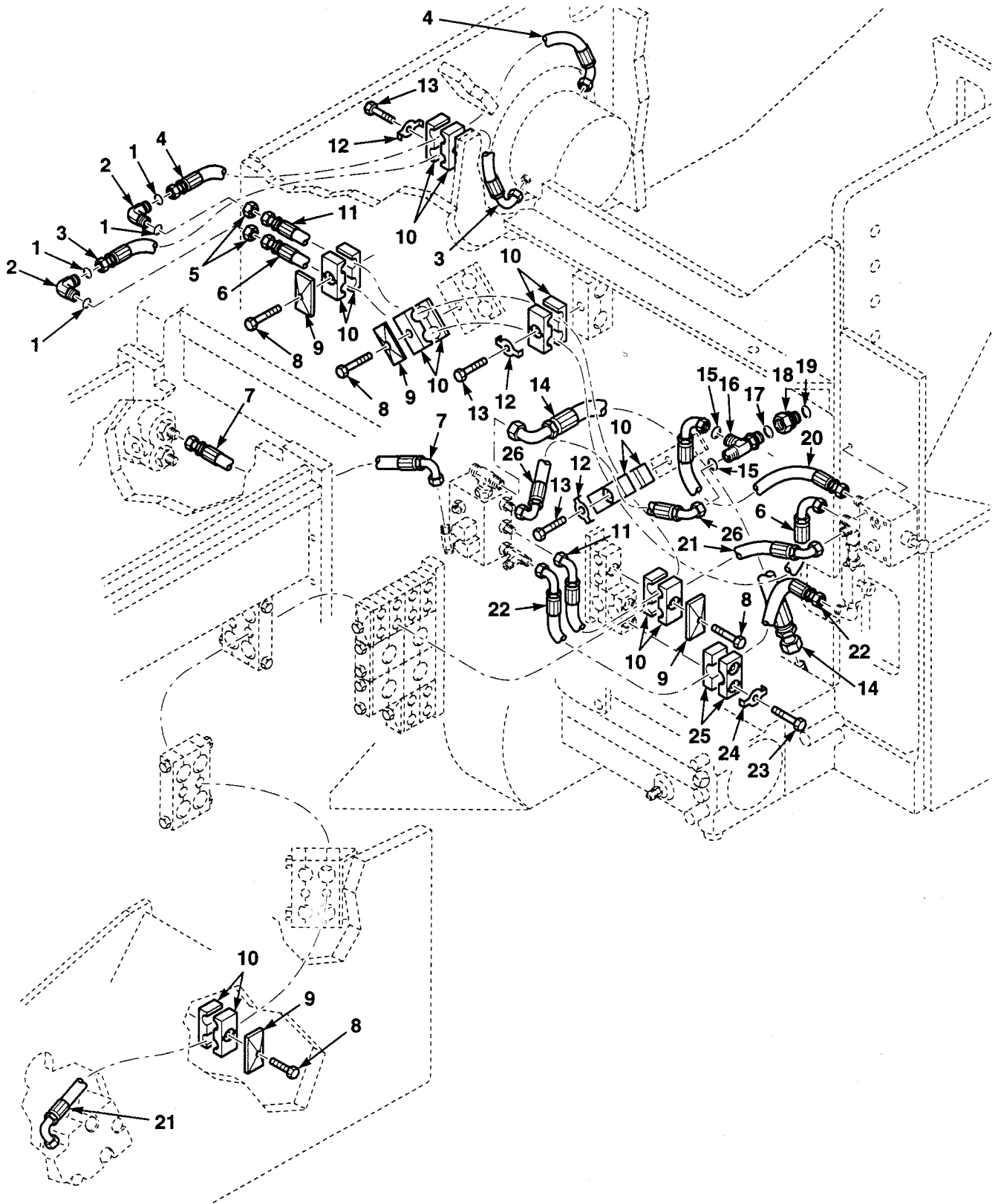
Figure 83. Brake Lines and Fittings
